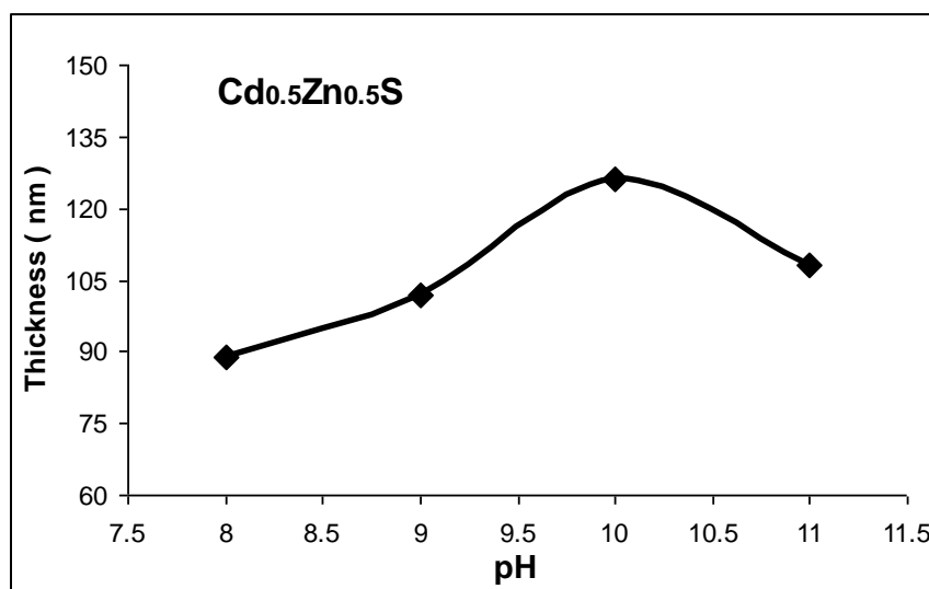
Figure (1) Influence of pH on \text{Cd}_{0.5}\text{Zn}_{0.5}\text{S} film thickness.
