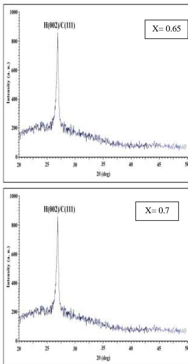
Figure (4) shows the X-ray diffraction for \text{Cd}_{1-x}\text{Zn}_x\text{S} thin films for different Zn- content ( x = 0, 0.2, 0.35, 0.5, 0.65, 0.7 ) after annealed at 300^\circ\text{C} for 1h.
