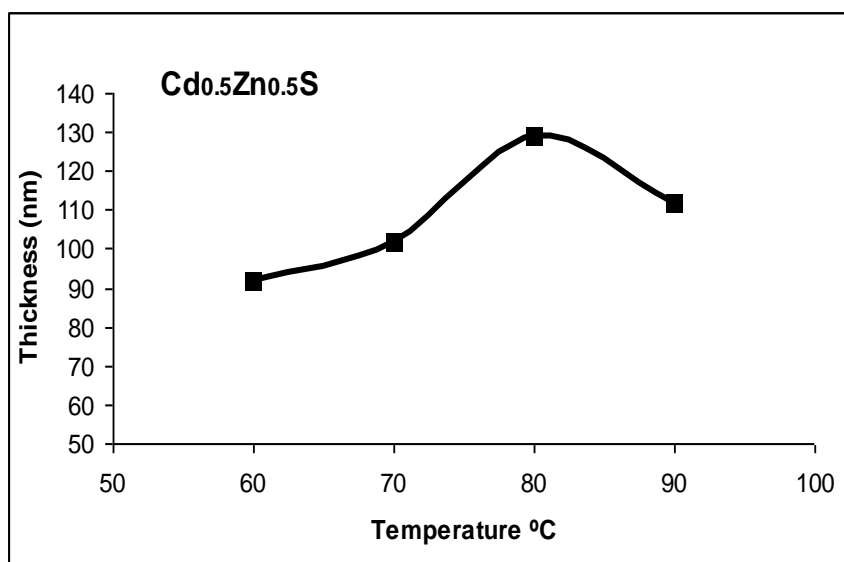
Figure (3) \text{Cd}_{0.5}\text{Zn}_{0.5}\text{S} film thickness dependence on bath temperature.
