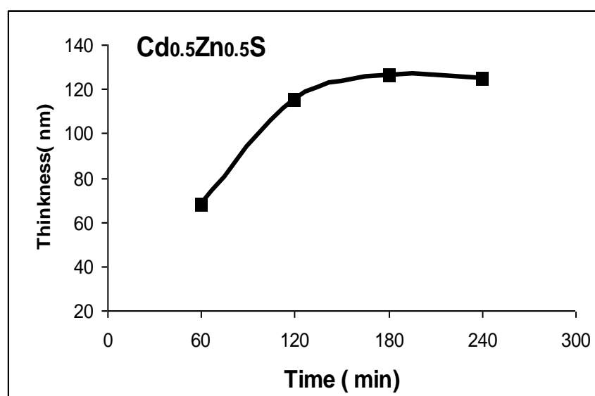
Figure (2) Thickness of \text{Cd}_{0.5}\text{Zn}_{0.5}\text{S} thin film as a function
