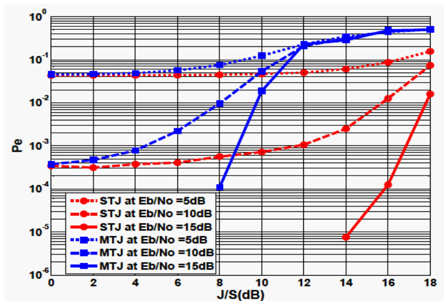
Figure (15) The P_e versus J/S for different E_b/N_0 for DS at k=24 dB with STJ and MTJ.
