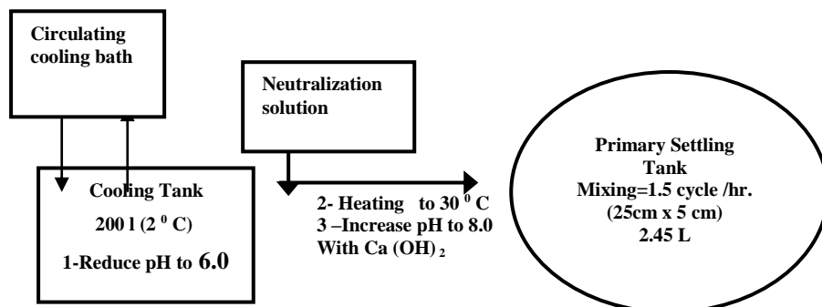
Figure (1) the diagram of laboratory scale construction of T2 line in Alrustamyia station for wastewater treatment.
