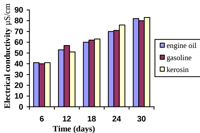
Fig.4. Electric conductivity of consortium after 30 days o growth
