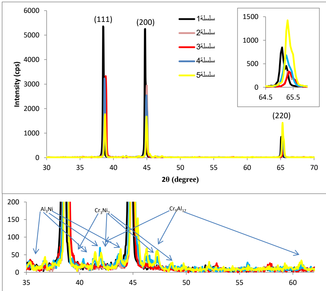
Fig. 3 :XRD pattern of Al and Al-Ni-Cr alloys.
