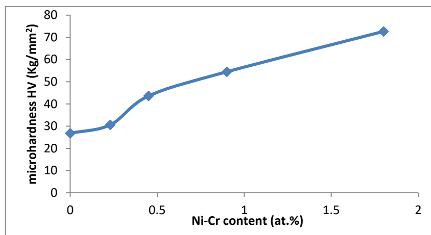
Fig. 5: Effect of content Ni-Cr at.% on Vickers microhardness of aluminum.
