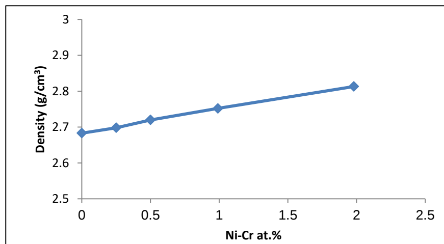
Fig. 4: Effect of content Ni-Cr at. % on density of aluminum alloy.
