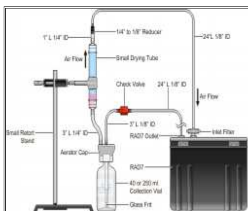
Fig.(2) Schematic presentations of radon-in-air monitor RAD7. Adapted from reference with permission [8]
