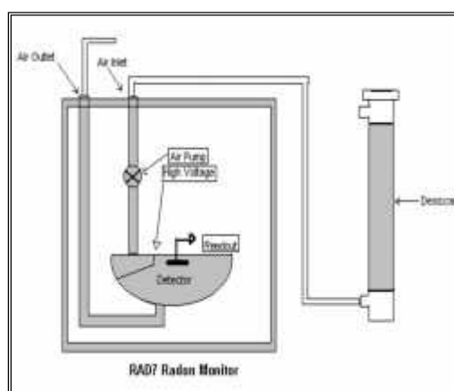
(Figure 3) Device scheme of RAD7 [9]
