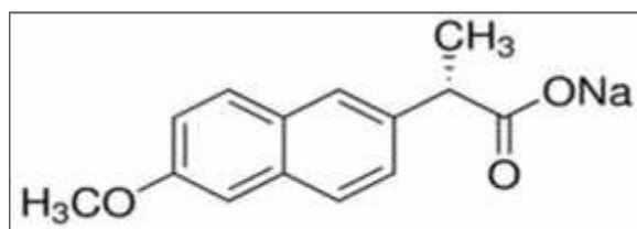
Figure (4) Structure of Naproxen Sodium
