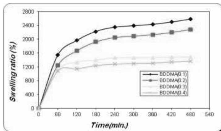
Figure(9) swelling ratio of cross-linking PAA-PVP copolymer hydrogels vs. time at pH=4
