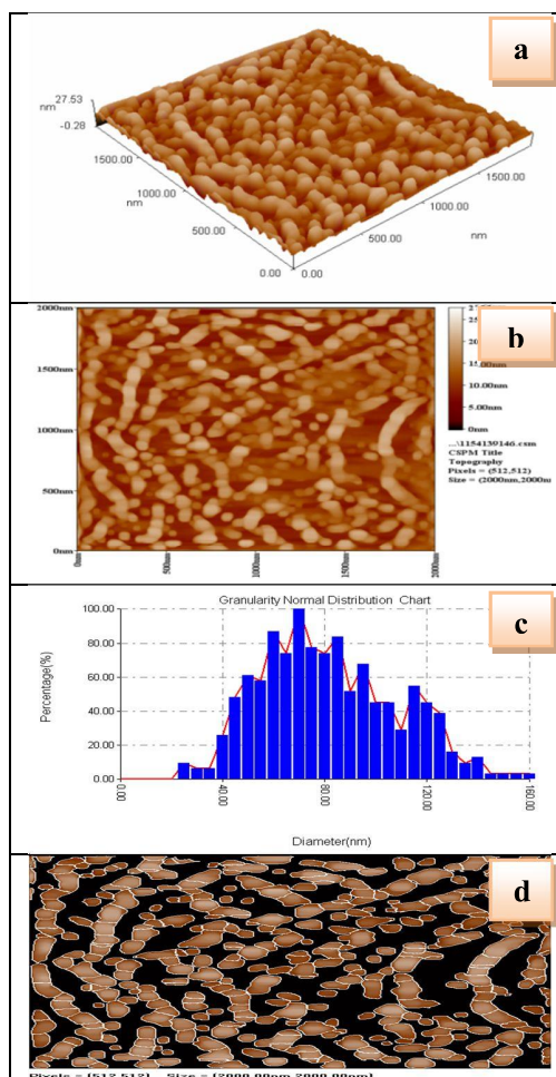
Fig.(2): AFM images of CdO thin film.
