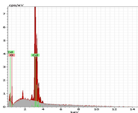
Fig. (4): EDX spectra of the CdO thin film.
