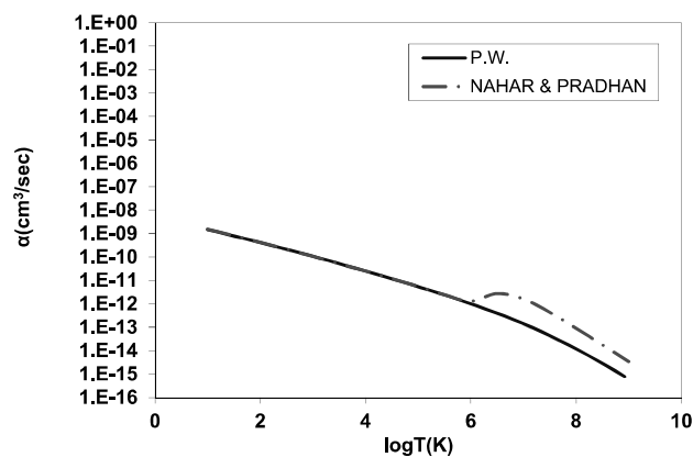
FIG(5):THE SAME AS IN FIG(4), EXCEPT FOR (N VI)-ION
