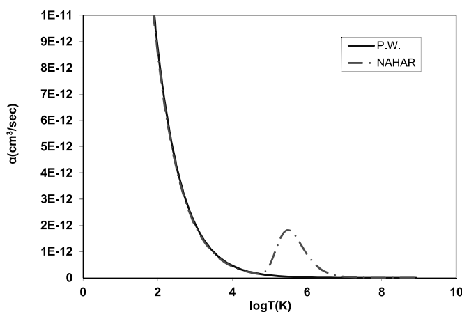
FIG(2):RADIATIVE RECOMBINATION RATE OF (He I)- ION. THE PRESENT WORK(P.W.) COMPARED WITH NAHAR.
