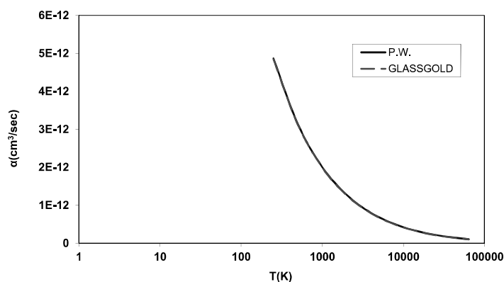
FIG(1):RADIATIVE RECOMBINATION RATE OF (H I)-ION. THE PRESENT WORK(P.W.) COMPARED WITH GLASSGOLD.
