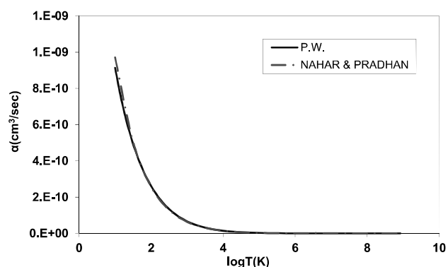
FIG(4):RADIATIVE RECOMBINATION RATE OF (N V)-ION. P.W. COMPARED WITH NAHAR & PRADHAN.
