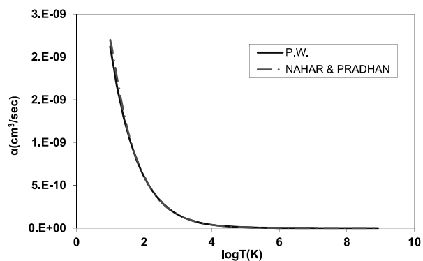
FIG(6):THE SAME AS IN FIG(4), EXCEPT FOR (N VII)-ION
