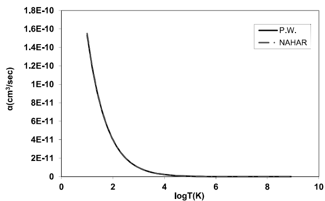
FIG(3):THE SAME AS FIG(2), EXCEPT FOR (He II)-ION.
