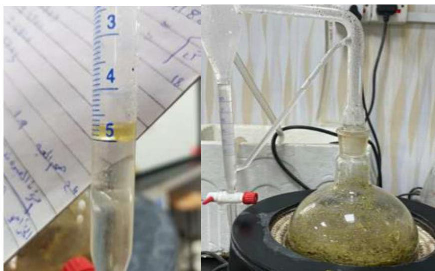
Figure 3: Clavenger Device for Extracting Essential Oil
