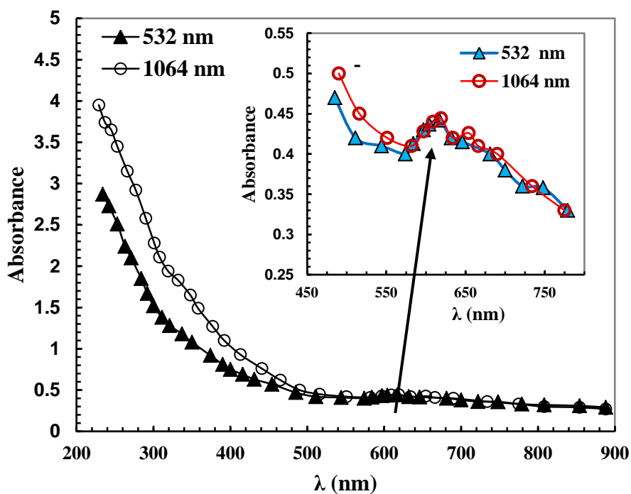
Figure (3) Absorbance spectra of the CuO nanoparticles, obtained by laser ablation of copper plates immersed in pure water exposed by 200 laser pulses, with laser fluence of 46 \text{ J/cm}^2 , at laser wavelength of 1064 nm and 532 nm, respectively.
