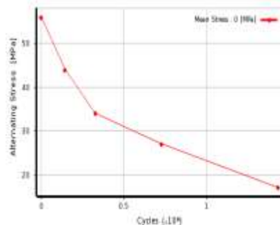
E: (S-N) curve for (9 Layers)
