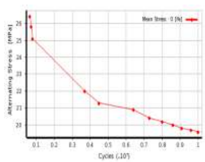
C: (S-N) curve for (PP)
