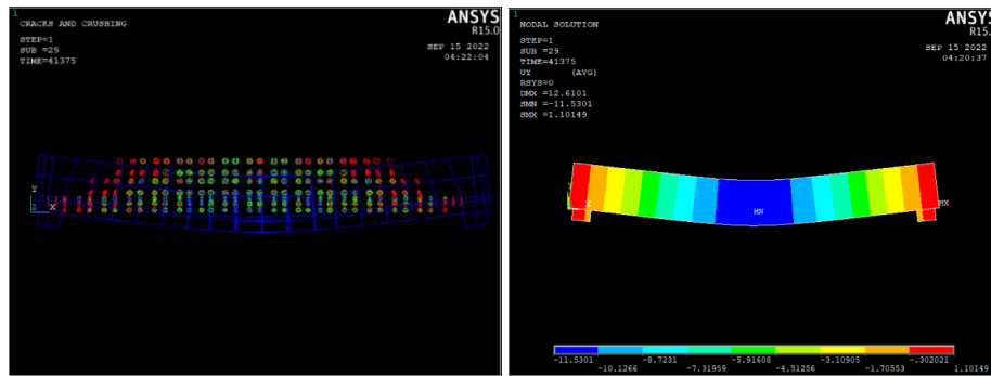
k. Crack pattern and deflection of HFRS-1 slab specimen Figure 4 Cracks pattern and deflection of slabs by ANSYS program
