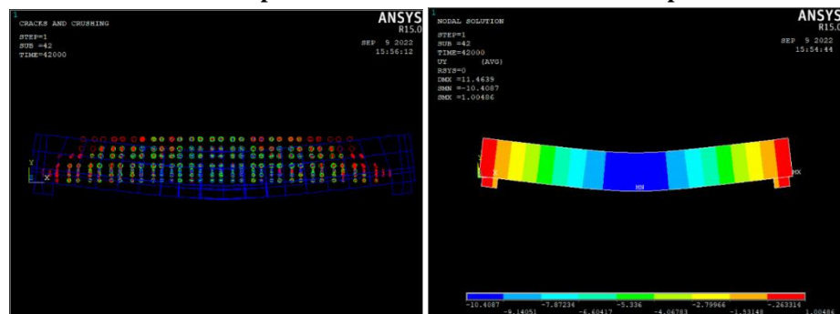
h. Crack pattern and deflection of PFRS-1 slab specimen
