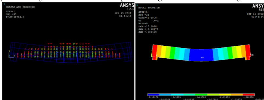
a. Crack Pattern and deflection of FRC-0 slab specimen
