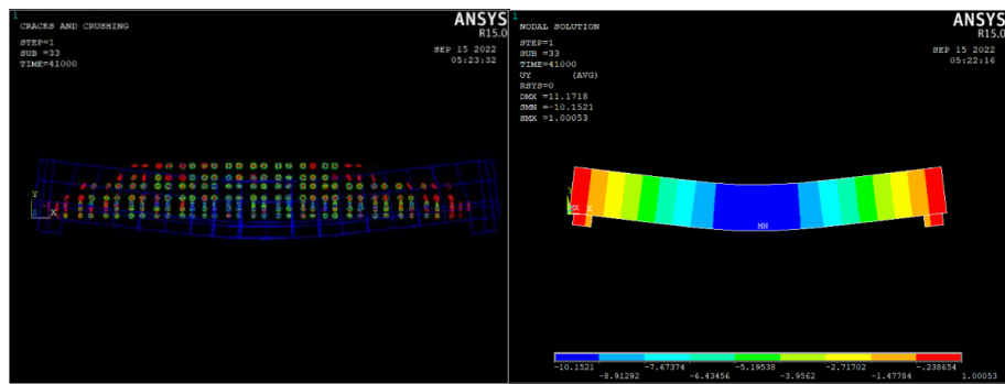
c. Crack pattern and deflection of WFRS-0.35 slab specimen
