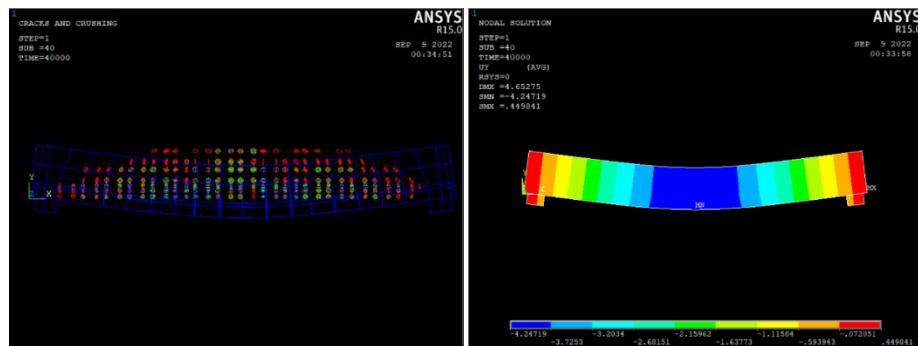
c. Crack pattern and deflection of WFRS-0.35 slab specimen
