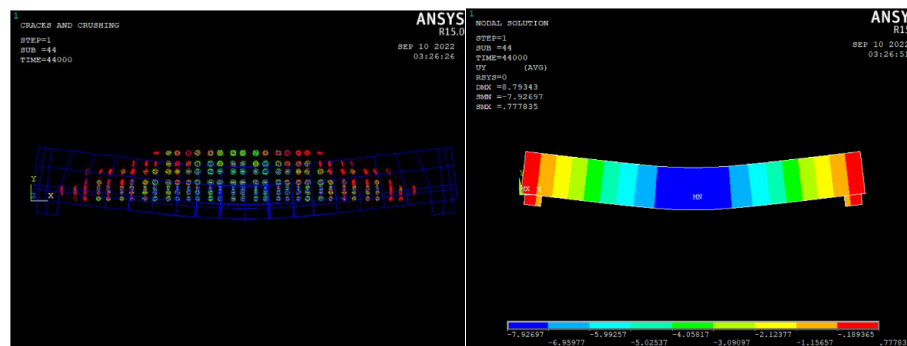
f. Crack pattern and deflection of PFRS-0.35 slab specimen
