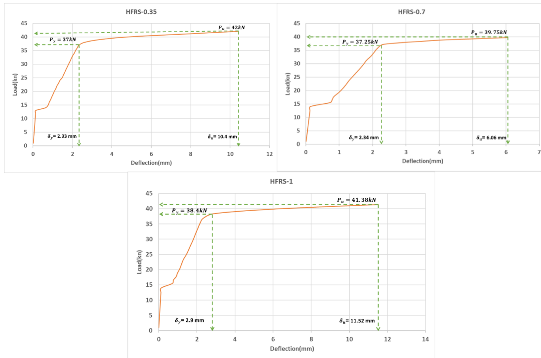
d. load- deflection curve of Slabs for Group-4
