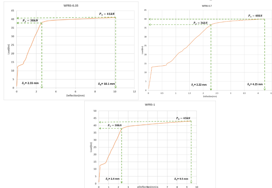
b. Load- deflection curve of Slabs for Group-2
