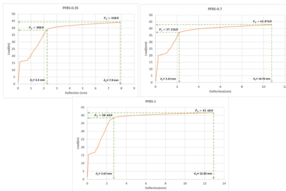
c. Load- deflection curve of Slabs for Group-3
