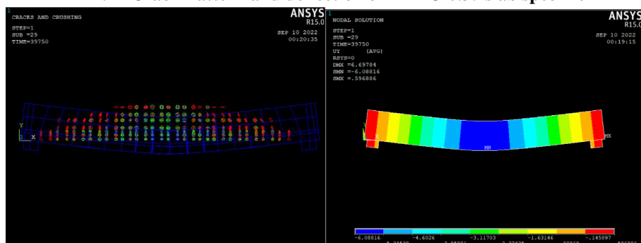
i. Crack Pattern and deflection of HFRC-0.35 slab specimen
