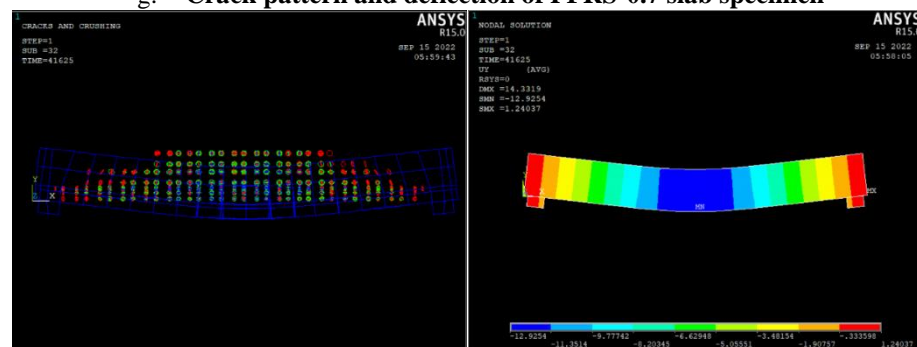
g. Crack pattern and deflection of PFRS-0.7 slab specimen
