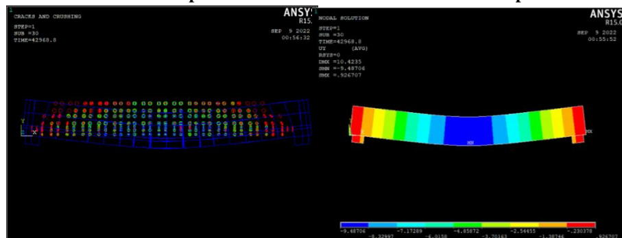
d. Crack pattern and deflection of WFRS-0.7 slab specimen
