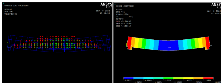
b. Crack pattern and deflection of FRS-0 slab specimen
