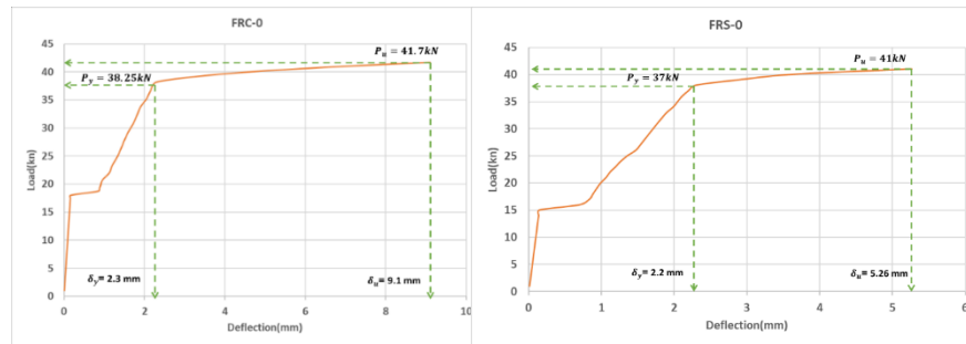
a. Load- deflection curve of Slabs for Group-1
