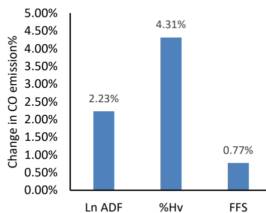
Fig. 5 Estimated elasticity effects of a 10% increase in Ln ADF, HV% and FFS on Co emission
