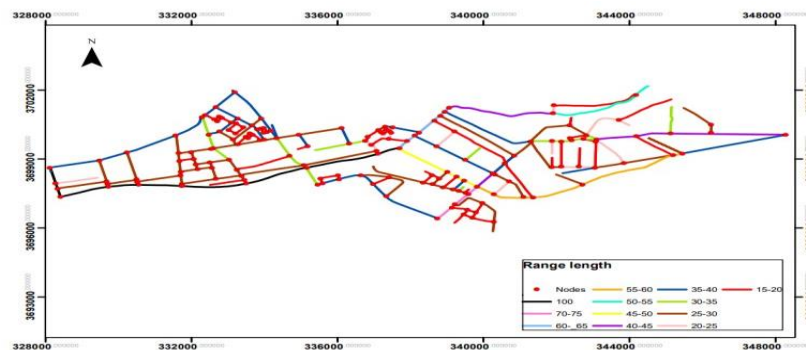
Fig. 1 Selecting arterial roads in the Ramadi road network
