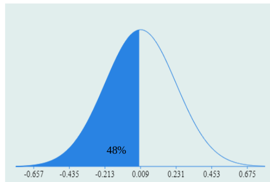
Fig. 3 Estimation of the distribution for %HV parameters for CO emission model
