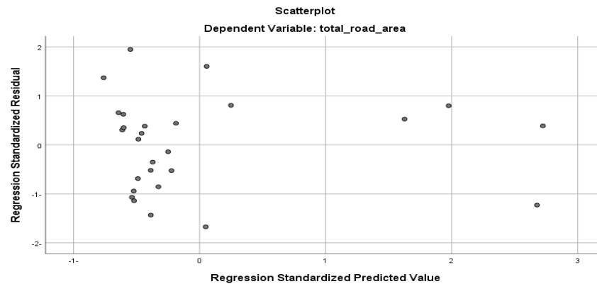
Figure 7. Scatter plot
