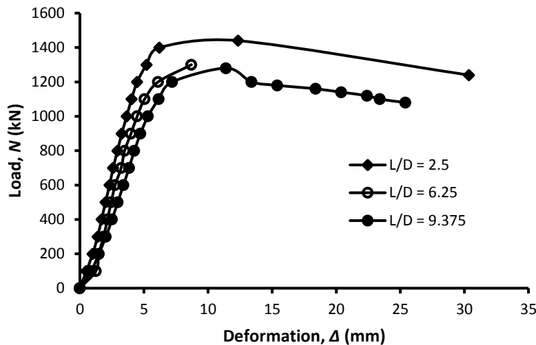
Figure. 8 Load-deformation behavior
