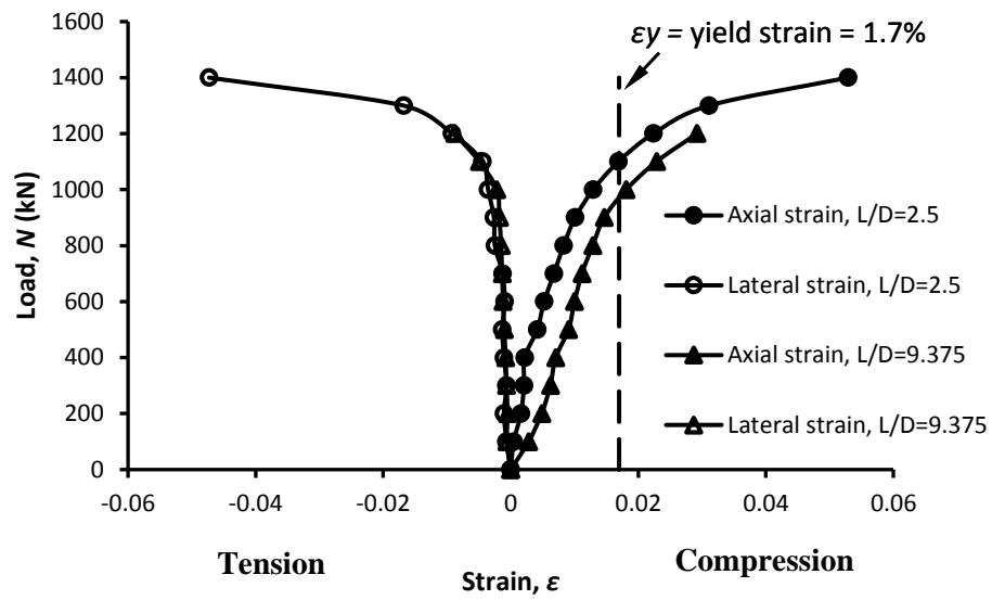
Figure. 9 Load-strain relationship
