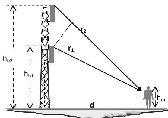
Figure 3. Effect of Antenna Height Height Relation
