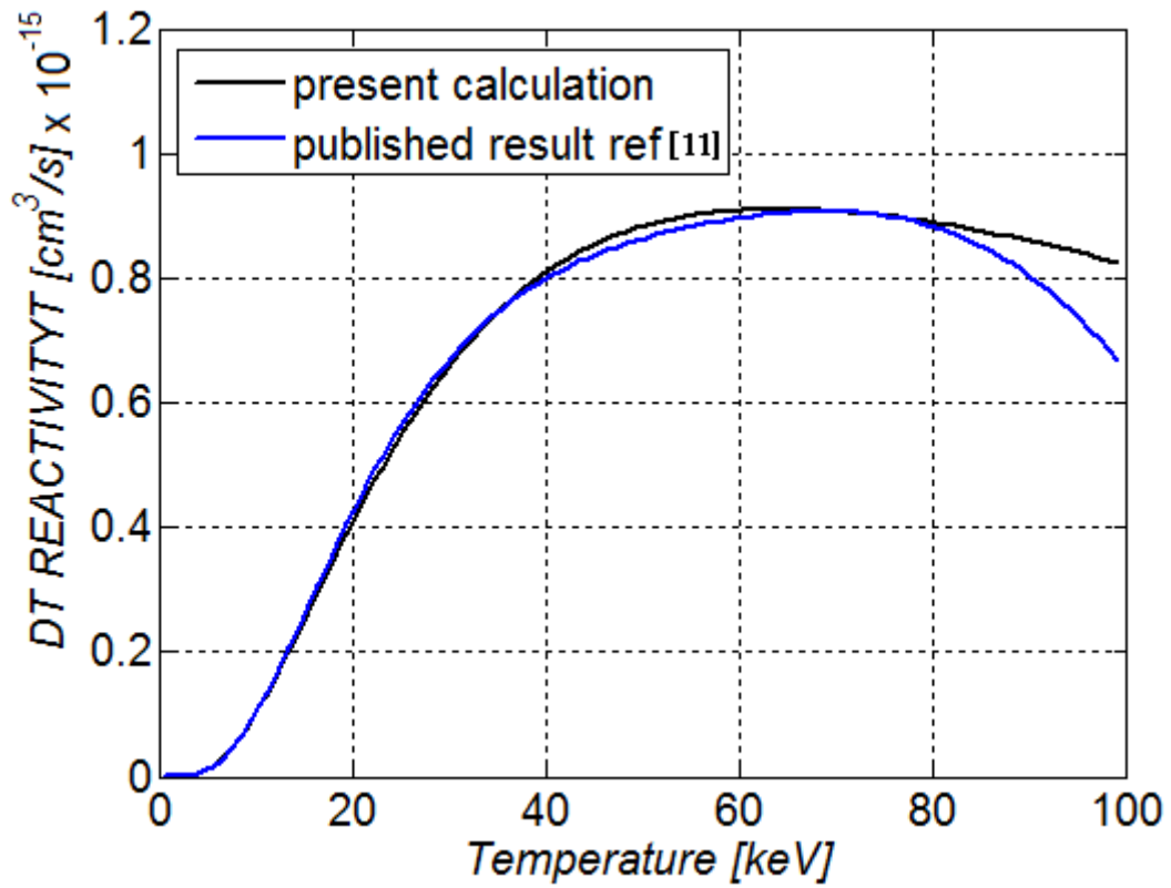
Figure 3. Variation of the D-T Reactivity versus the incident deuteron temperature
