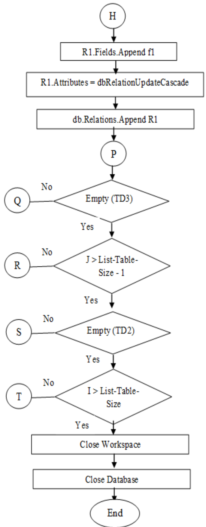
Figure 11. 1: N Relationship.
