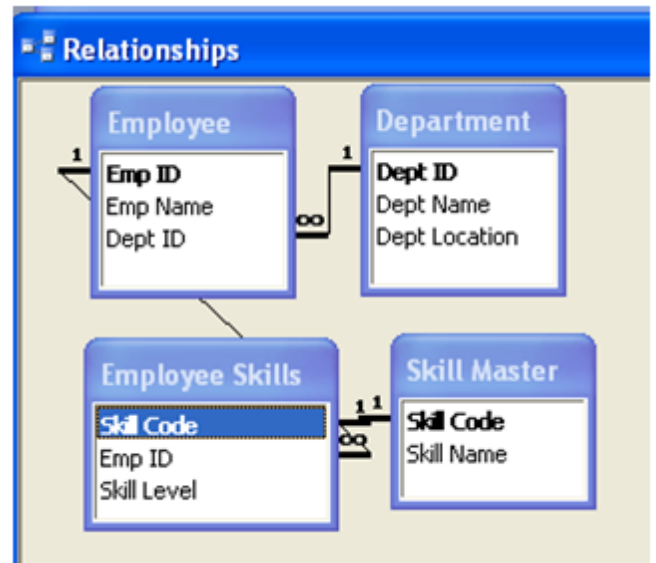
Figure 15. Creating Relationship between Tables.
