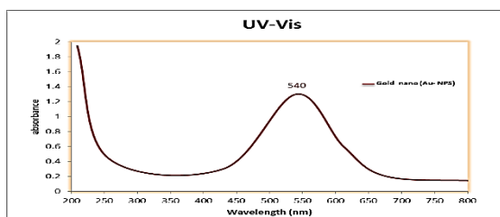
Fig. 2: The absorption spectrum of gold nanoparticles manufactured by Lion's mane mushroom extract.
