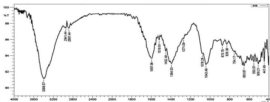
Fig. 4: The absorption spectrum of gold nanoparticles biosynthesized by Lion's mane mushroom extract using an FTIR device.
