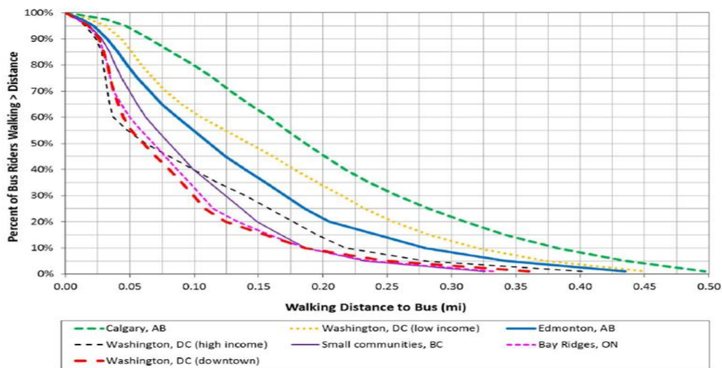
Figure 1: Walking distance to bus stops (Source: TCQSM, Report 165, Ch. 4, P.18)
