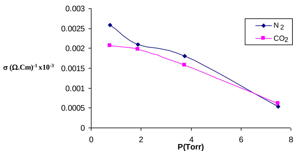
Fig (7) The relation between conductivity and pressure of N 2 and CO 2 gases
