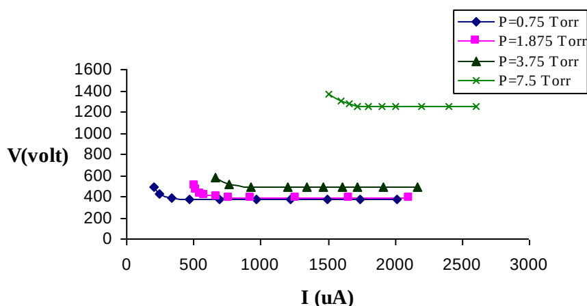
Fig (5) The (V-I) measurement at different Pressure for CO_2
