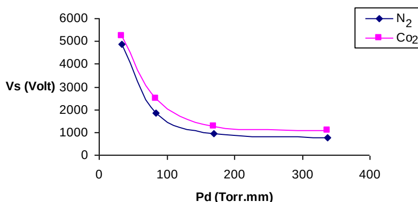
Fig (3) The sparking potentials in N_2 and CO_2 gases as a function of (pd)
