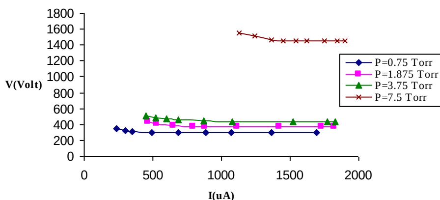
Fig (4) The (V-I) measurement at different Pressure for N_2
