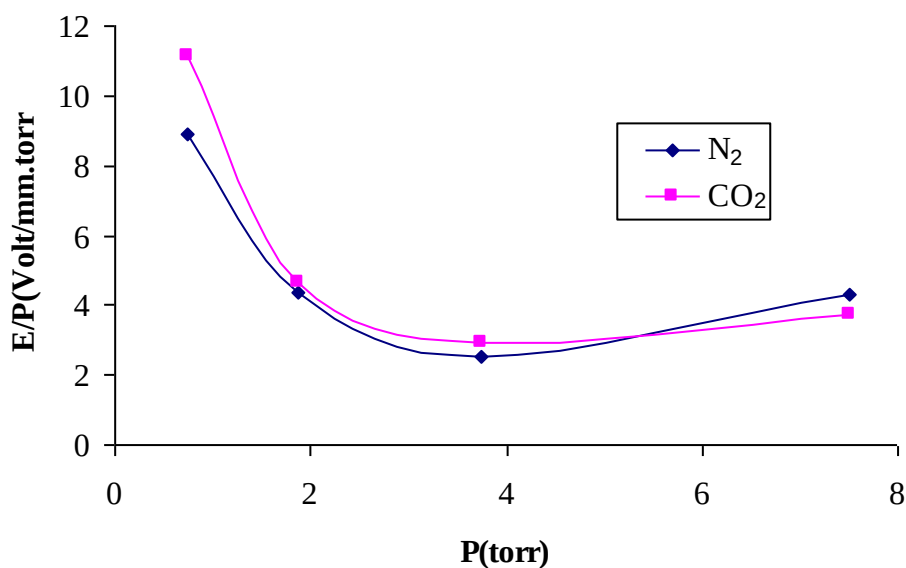
Fig (6) The relation of (E/P) with (P) for CO 2 and N 2 gases
