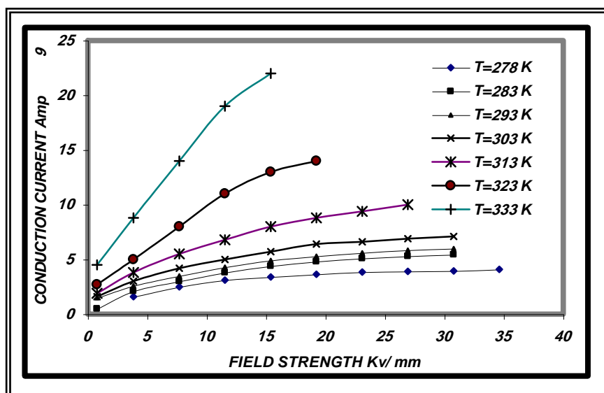
Figure (3) The conduction current as a function of applied electric field at different temperature in n-hexane
