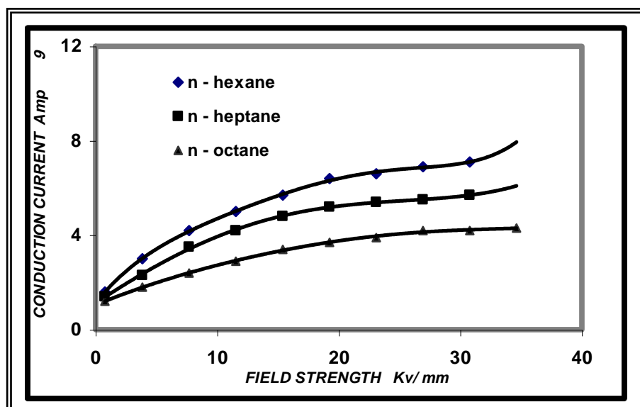
Figure (2) The conduction current as a function of applied electric field at different saturated hydrocarbon liquids (T=303 oK)
