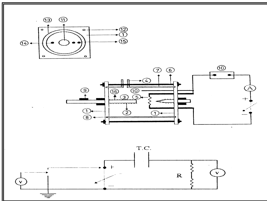
Figure(1): Experimental apparatus (Schematic diagram of the test cell and electrical circuit. A-Ammeter R-Standard Resistor V-Voltmeter 1-Teflon base 2- Brass needle electrode 3-Brass plane electrode 4-Filling port 5-Heater 6-Steel fitting rod 7-Glass envelop 8-Gasket 9-Brush 10-Temperature control 11-Electrode fitting hole 12-Rod fitting hole 13-Test cell setting groove 14-Heater voltage connection 15-Temperature control hole 16-Insulation cover.
