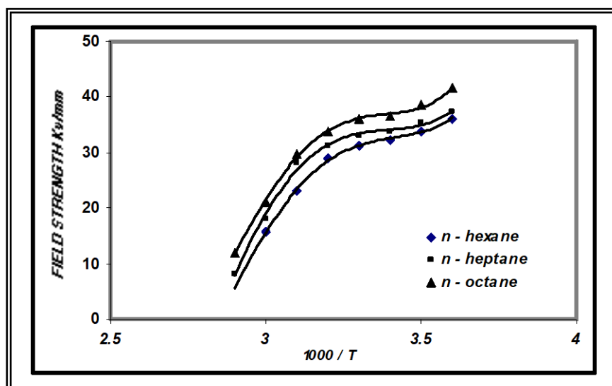
Figure (4) Temperature dependence on breakdown field strength for different saturated hydrocarbon liquids
