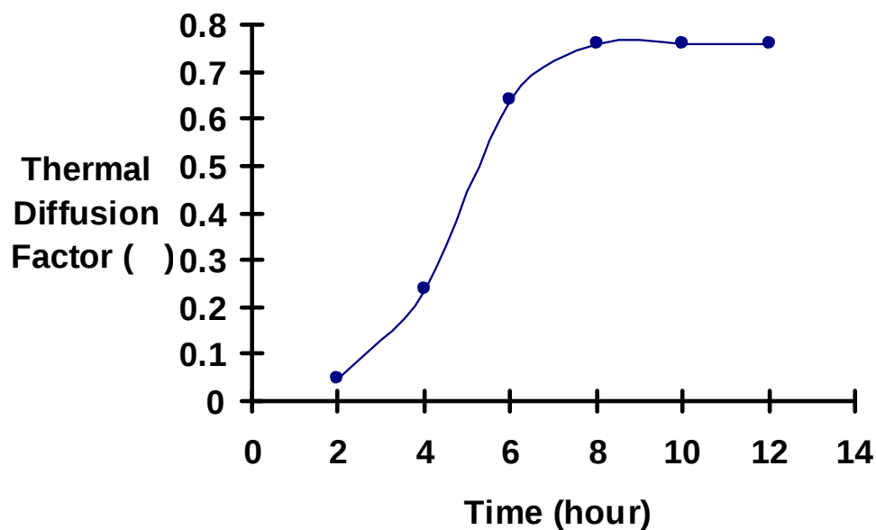
Fig.(3) : The relation between thermal diffusion factor and time
