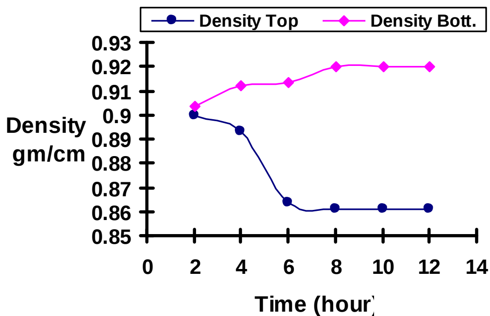
Fig.(4) : The relation between the densities of upper and lower samples with time
