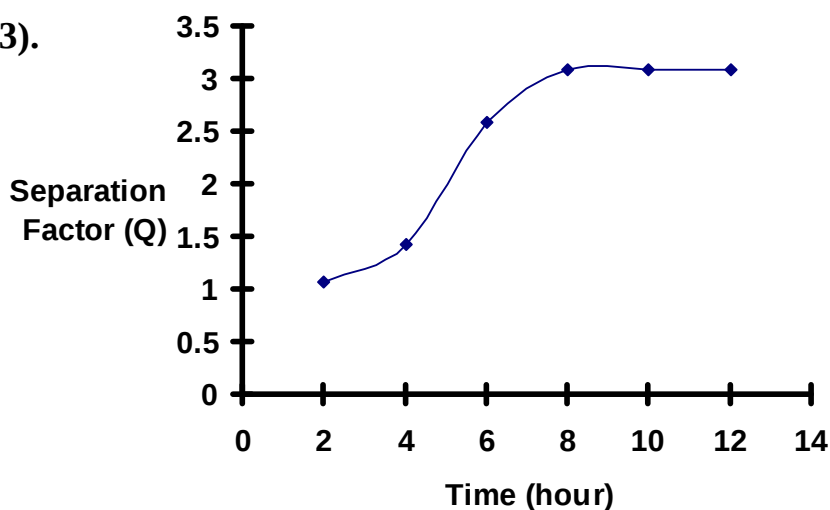
Fig.(2) : The relation between the separation factor and time
