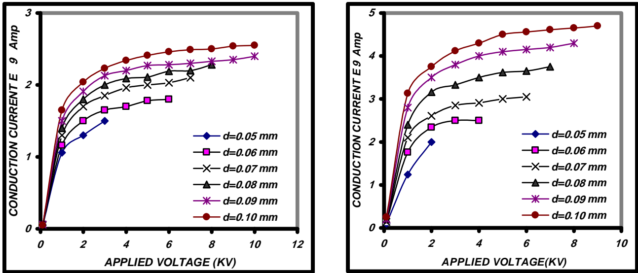
Figure(2): Typical graph of current voltage characteristics in n pentane under the influence of convergent field conditions for Ag and Al respectively
