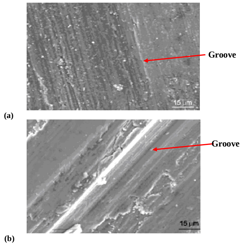
Figure (9) Worn surface morphology of Al-Si/ \text{Al}_2\text{O}_3 composites (a)squeeze cast (b)stir processed
