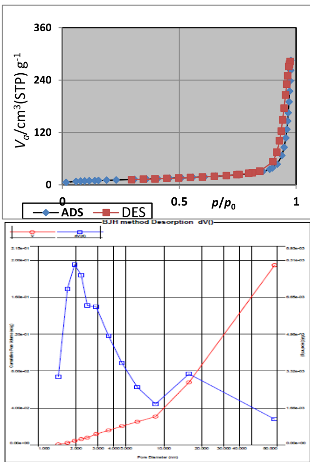
Fig. 6. a: N 2 adsorption-desorption isotherm, b: distribution of the pore size of ch-MPS.
