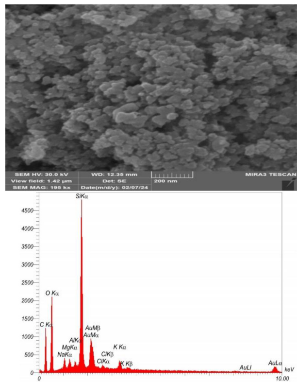
Fig. 5. SEM pictures and EDX spectrum of gr-SiO 2 .
