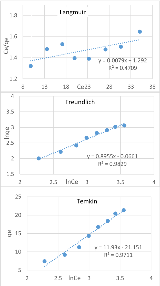
Fig. 9. Linear plots for the three models at 303 K for adsorption of amlodipine drug on gr-SiO 2 .
