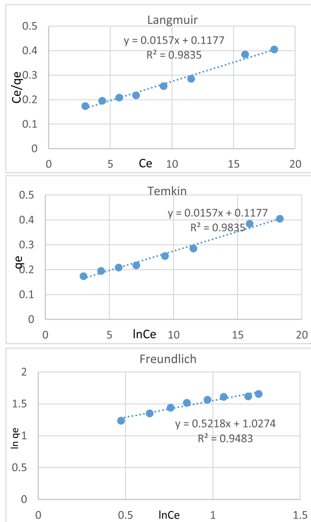
Fig. 8. Linear plots for the three models at 303 K for adsorption of amlodipine drug on ch-SiO 2 .
