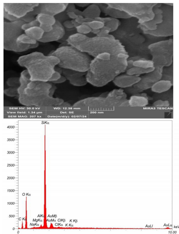
Fig. 4. SEM pictures and EDX spectrum of ch-SiO 2 .
