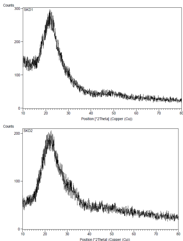
Fig. 2. Wide-angle XRD patterns of a: ch-SiO 2 , b: gr-SiO 2 .
