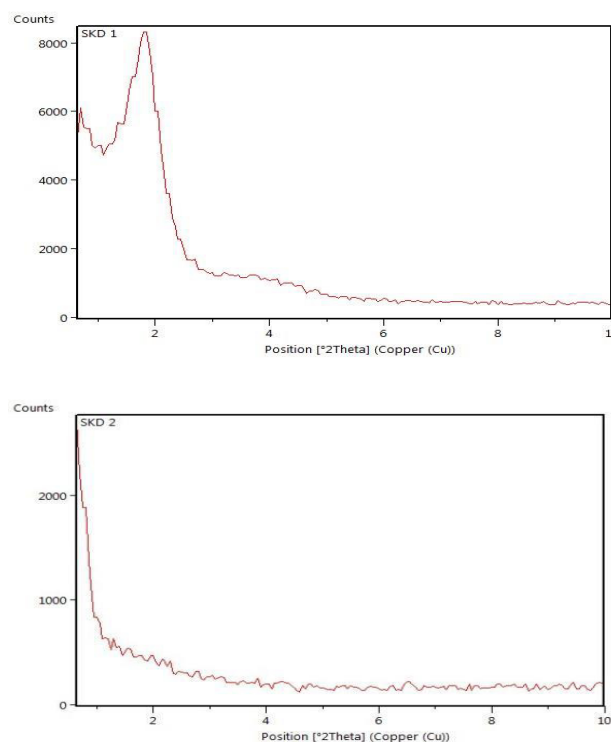
Fig. 3. Small-angle XRD patterns of a: ch-SiO 2 , b: gr-SiO 2 .
