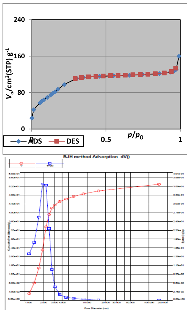
Fig. 7. a: N 2 adsorption-desorption isotherm, b: distribution of the pore size of gr-SiO 2 .
