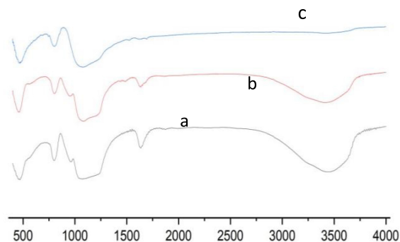
Fig. 1. FTIR spectrum of a: ch-SiO 2 before calcination, b: gr-SiO 2 before calcination, c: SiO 2 after calcination.
