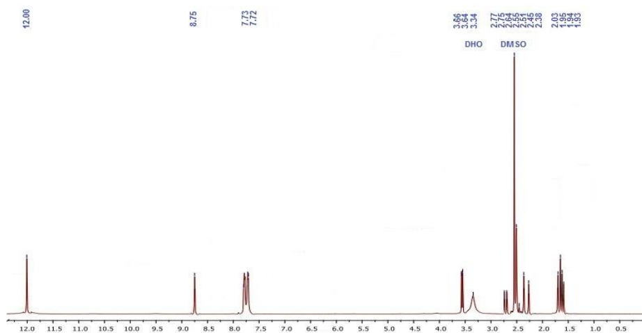
Figure 1: ^1\text{H} -NMR spectrum of ligand
