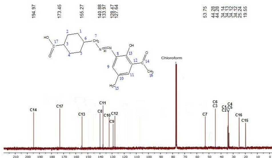
Figure 2: ^{13}\text{C} -NMR spectrum of ligand
