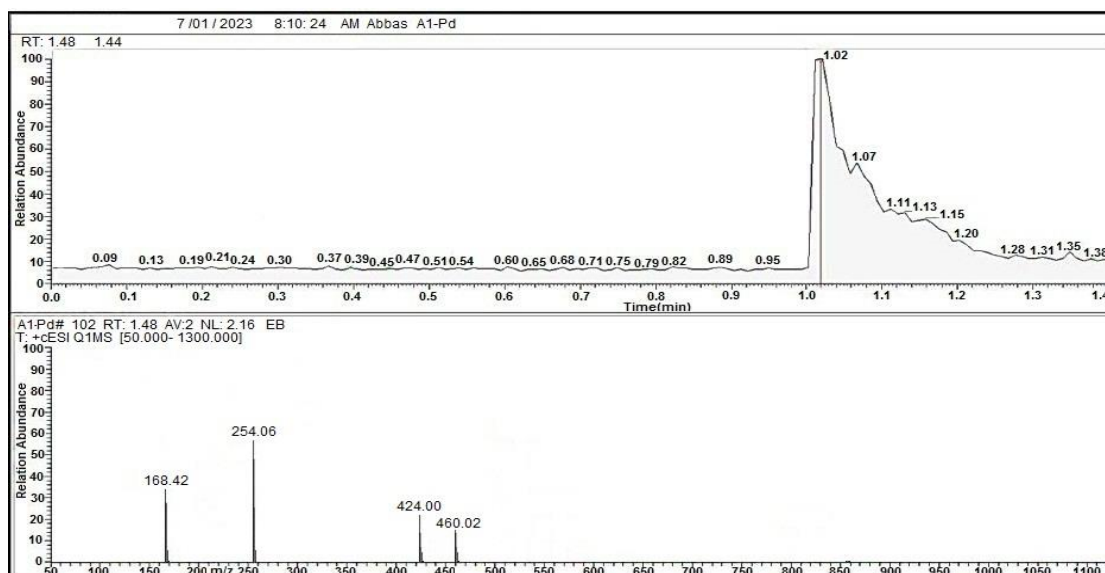
Figure 9: LC-Mass spectrum of Pd- complex
