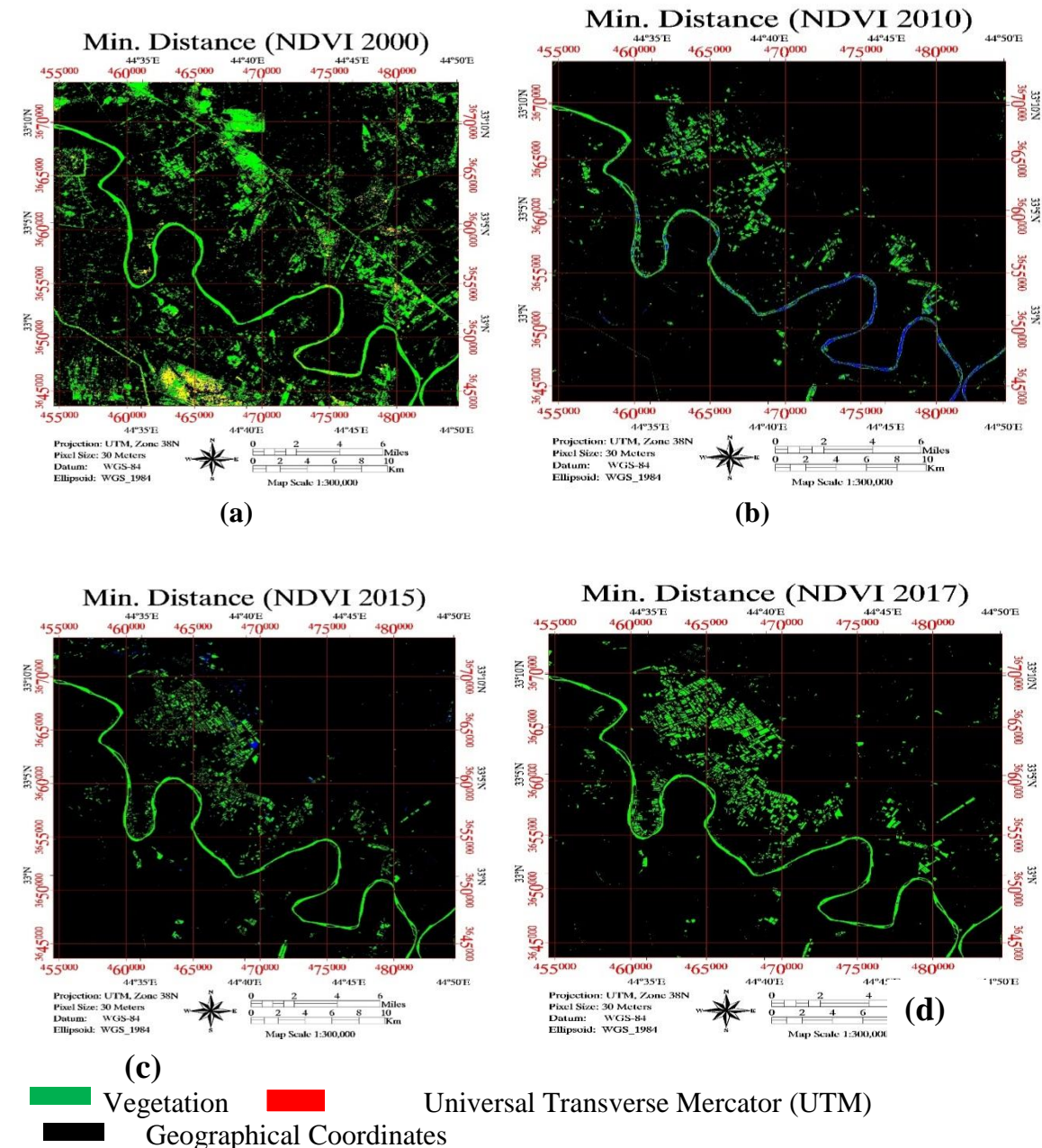
Figure 4- Minimum Distance Classification NDVI distribution in (a) 2000, (b) 2010, (c) 2015, and (d) 2017
