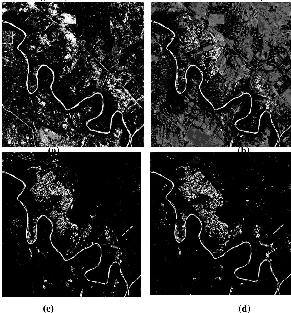
Figure -3 The NDVI distribution in (a) December 2000, (b) December 2010, (c) December 2015, and (d) December 2017
