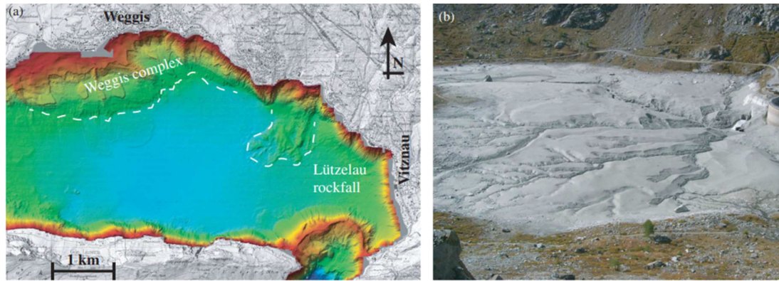
Fig. 4. (a) Vitznau basin of lake Lucerne where the Lützelau subaerial rockfall and the Weggis complex of subaqueous slides are represented (b) Sedimentation in Turtmann dam, Switzerland [15].
