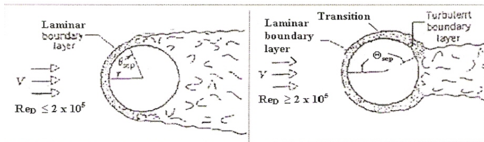
Figure (1) The Effect of Turbulence on Separation Around a Sphere [ Incropera 1996 ]
