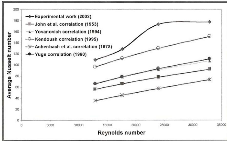
Figure (7) Relation Between Average Nusselt and Reynolds Numbers for Sphere Heated by Water at Temperature 70°C
