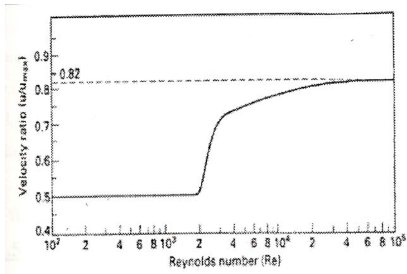
Figure (2) Variation of U/U_{\max} with Reynolds Number in a Pipe [Richarson 1996]
