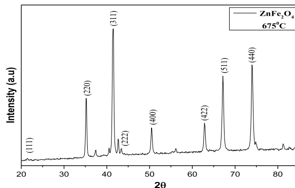
Fig. 5. XRD pattern of ZnFe 2 O 4 compound annealed at 675°C.
