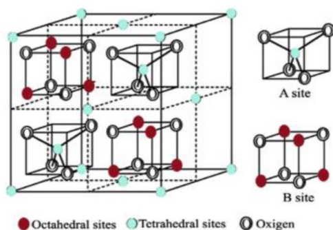
Fig. 1. The crystal structure of zinc ferrite 1 .
