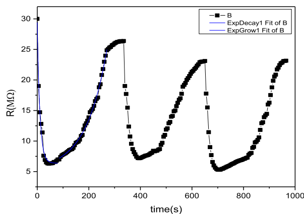
Fig. 10. The response curve as a function of time of ZnFe_2O_4 sensor on consecutive exposure to 100 ppm ethanol vapor with 3 cycles at 275°C (Reproducibility).
