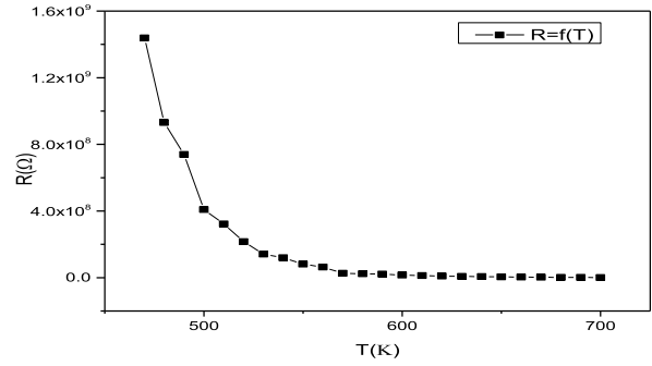
Fig. 7. Electrical resistance variations of ZnFe 2 O 4 compound as a function of temperature.
