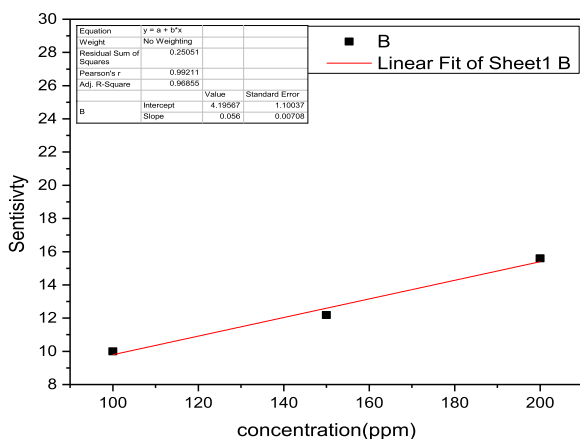
Fig. 15. The sensitivity as a function acetone vapor concentrations.
