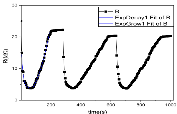
Fig. 11. The response curve as a function of time of \text{ZnFe}_2\text{O}_4 sensor on consecutive exposure to 100 ppm acetone vapor with 3 cycles at 300^\circ\text{C} (Reproducibility).
