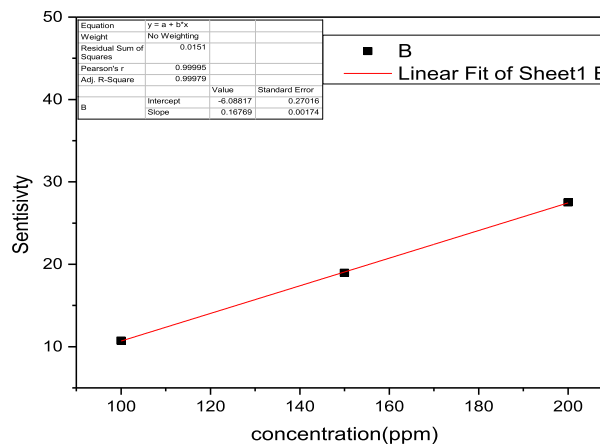
Fig. 14. The sensitivity as a function ethanol vapor concentrations.
