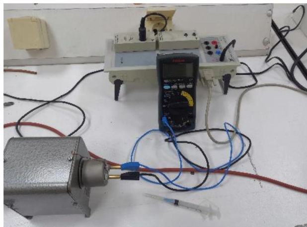
Fig. 2. The electrical measurement device.
