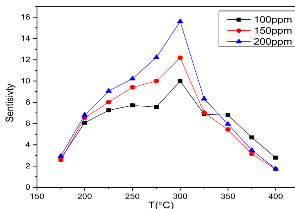
Fig. 13. The sensitivity curve as a function of temperature at different concentrations of acetone vapor.
