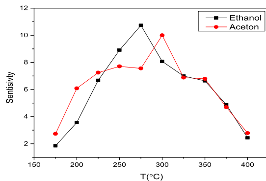
Fig. 9. Sensitivity of zinc ferrite nanoparticles to ethanol and acetone vapors at a concentration of 100 ppm.
