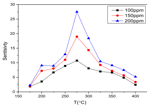
Fig. 12. The sensitivity curve as a function of temperature at different concentrations of ethanol vapor.
