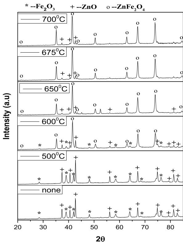
Fig. 4. XRD patterns of the prepared and annealed samples at different temperatures.
