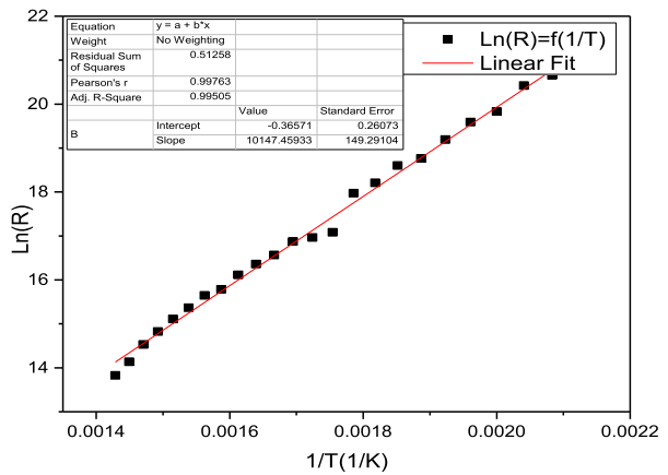
Fig. 8. Variation of ln(R) as a function of 1/T for ZnFe 2 O 4 compound.
