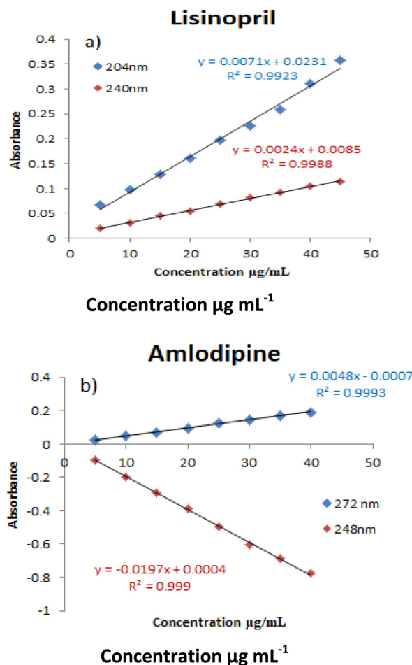
Fig. 5. (a) Calibration curve of LSD at 204 and 240 nm, (b) Calibration curve of AMD at 248, and 272 nm.
