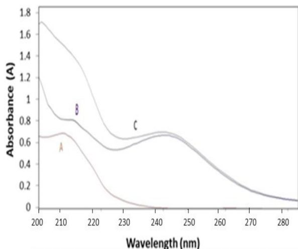
Fig. 2. Zero-order spectra of lisinopril (A), amlodipine (B), and amlodipine with lisinopril in 0.1 M HCl (C).
