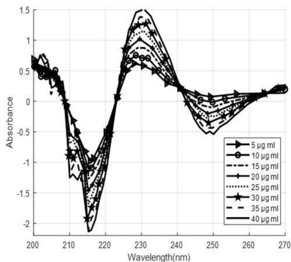
Fig. 3. Third derivative spectroscopy of various concentrations of amlodipine ( 5 \mu\text{g ml}^{-1} – 40 \mu\text{g ml}^{-1} ) Simultaneous Determination of Lisinopril and Amlodipine.
