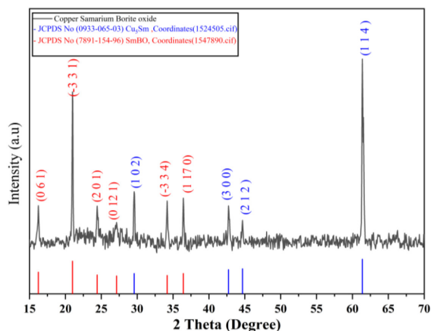
Fig. 2. XRD diffraction pattern of Copper Samarium Borate Oxide Nano composite thin film by hydrothermal method, annealed at 350°C.
