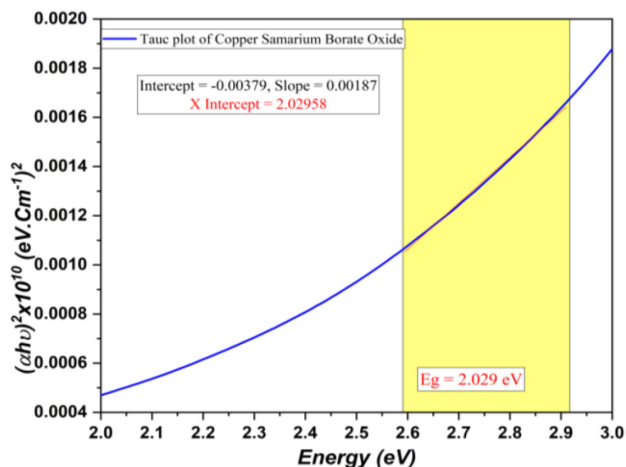
Fig. 5. Plotting the energy gap value of the allowed direct transmission of the prepared Copper Samarium Borate Oxide Nano composite thin film that annealing at 350°C for 3 hr.
