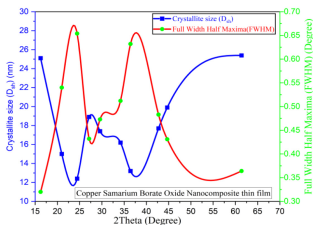
Fig. 3. Variation of crystallite size (Dsh), Full Width Half Maxima (FWHM) versus ( 2\theta ) of Copper Samarium Borate Oxide nanocomposite annealed 3 hours.
