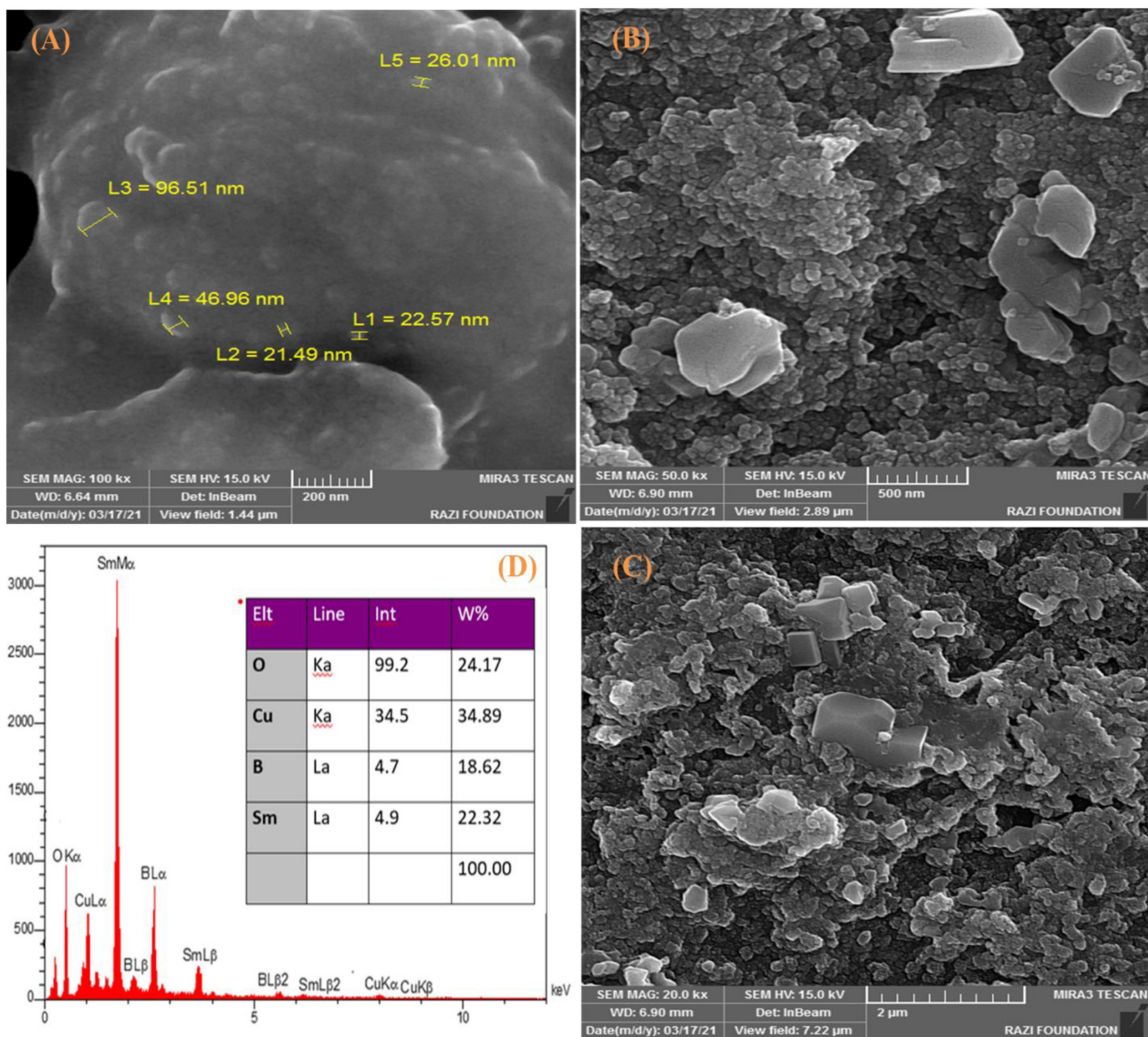
Fig. 1. SEM of Copper Samarium Borate Oxide CuSmBO nanoparticles composition thin film prepared by hydrothermal mechanism, that annealing at 350°C for 3 hr. (A, B and C) Surface morphology, ((A) high-resolution image), (B and C) inset: low-resolution image and magnification and (D) EDX analysis of CuSmBO nanoparticles composition thin film.
