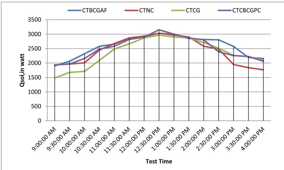
Fig. 8. The amount of heat entering the system using four different receiver surroundings, along with the measurement time.
