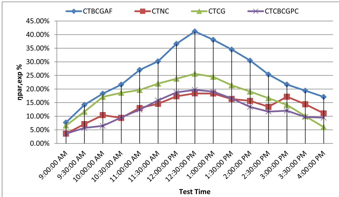
Fig. 11. The practical thermal efficiency using four different receiver surroundings, along with the measurement time.
