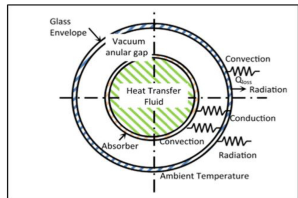
Fig. 6. Cross-sectional scheme of a PTC receiver for the Heat Transfer Mode. 27
