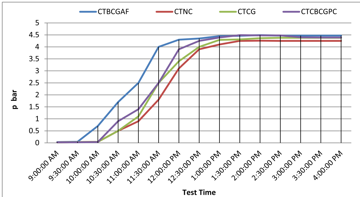
Fig. 12. The generated pressure inside the tank using four different receiver surroundings, along with the measurement time. for the data was averaged.
