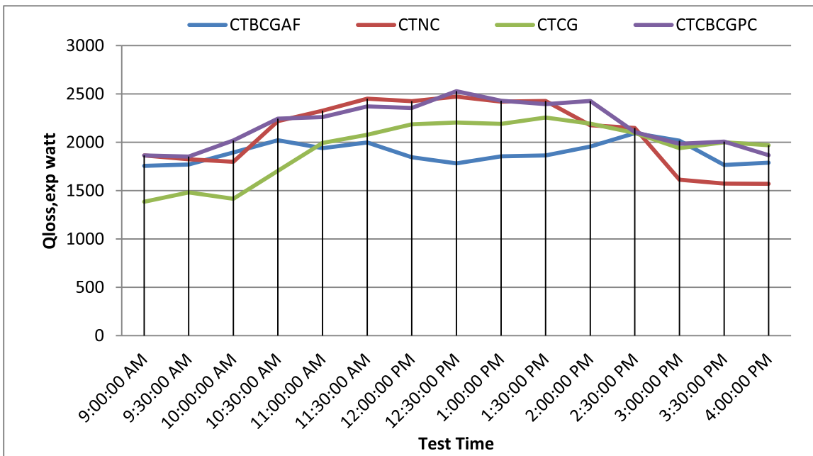
Fig. 10. The practical heat losses using four different receiver surroundings, along with the measurement time.
