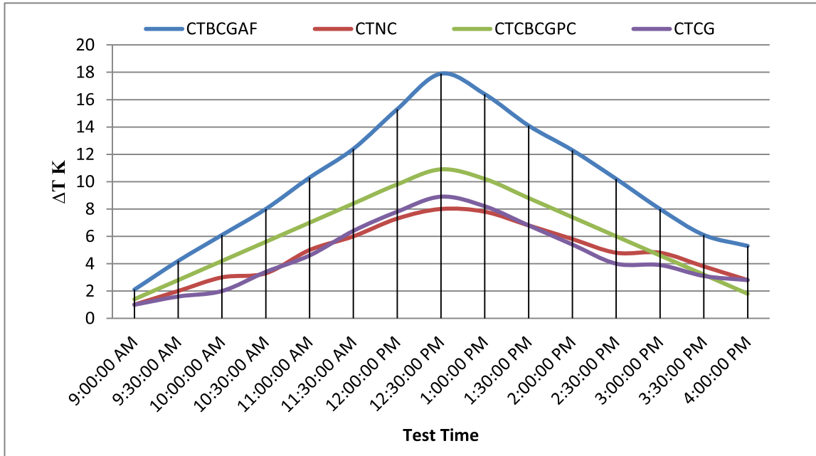
Fig. 7. The temperature difference between the inlet and outlet of the fluid using four different receiver surroundings, along with the measurement time.
