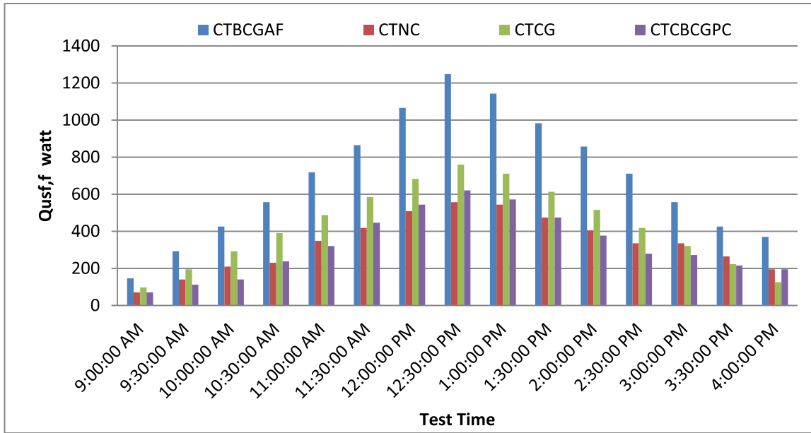
Fig. 9. The useful heat quantity obtained using four different receiver surroundings, along with the measurement time.
