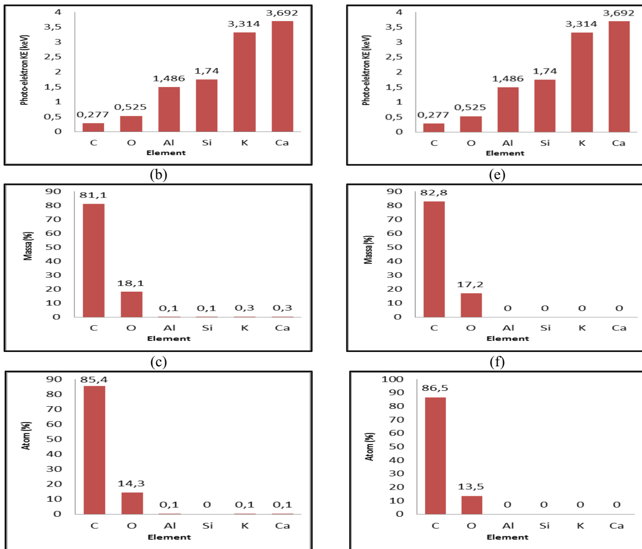
Fig. 5. Graph of (a) KE photo electrons, (b) % mass, (c) % atoms from pyrolyzed walnut shell carbon and (d) KE photo electrons, (e) % mass, (f) % atoms from KCl-activated walnut shell carbon.
