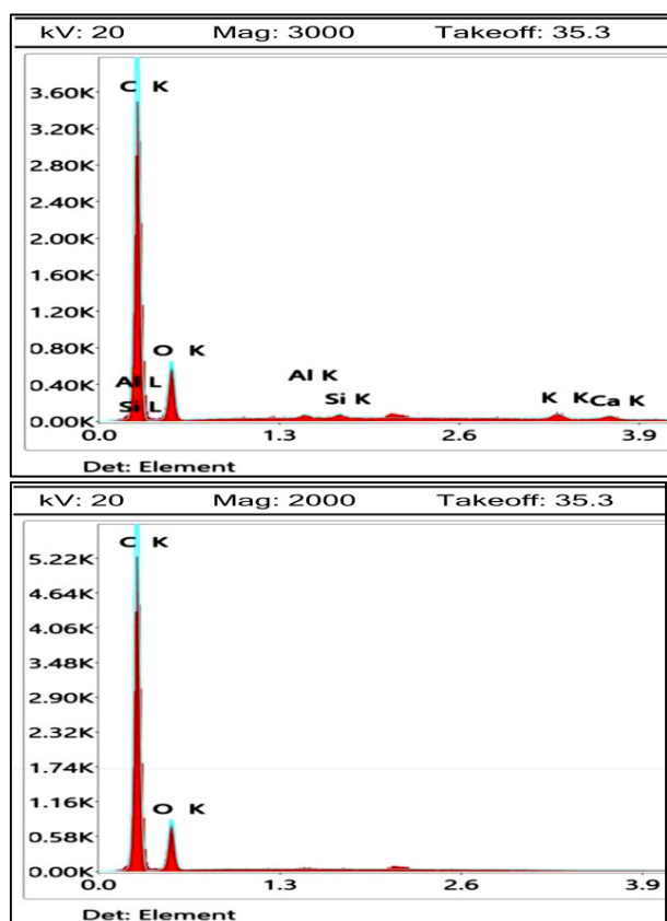
Fig. 4. EDX spectrum of pyrolyzed (a) and KCl-activated walnut shell carbon (b).
