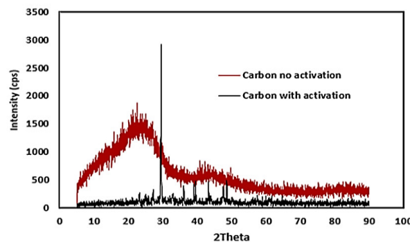
Fig. 6. Walnut shell carbon diffractogram resulting from pyrolysis (---) and diffractogram of walnut shell carbon after KCl activation (---).
