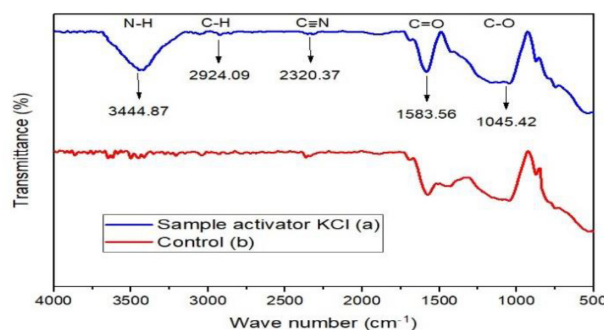
Fig. 1. FTIR spectrum of the walnut shell carbon after KCl activation (a) And before KCl activation (b).
