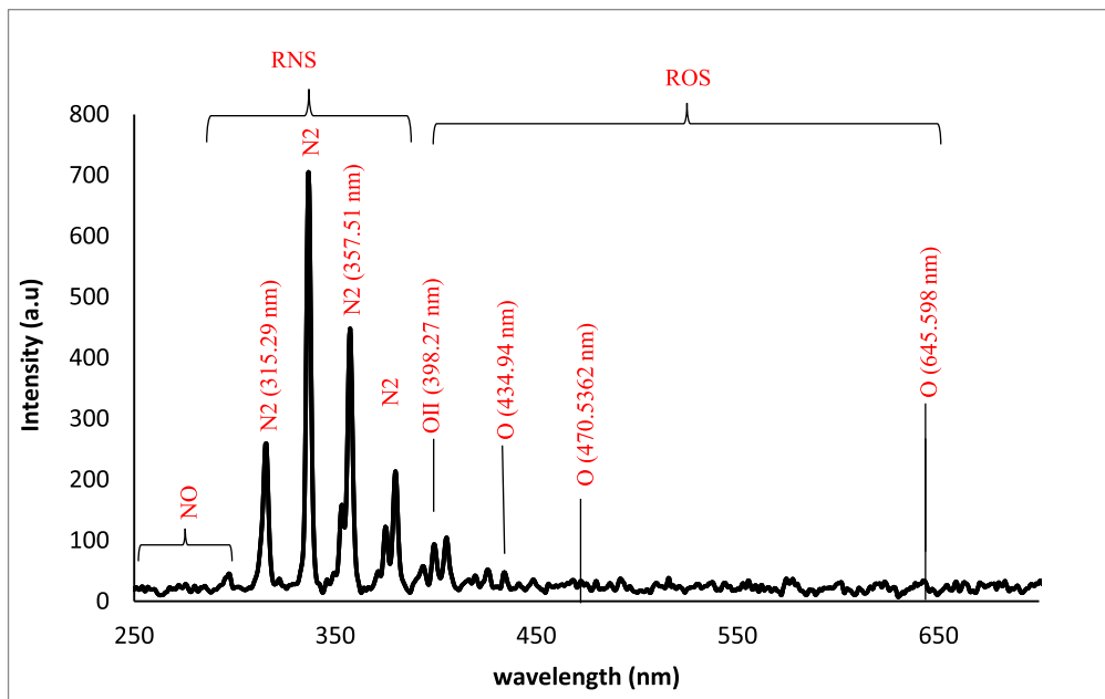
Fig. 5. Optical emission spectrum of cold plasma by DBD.
