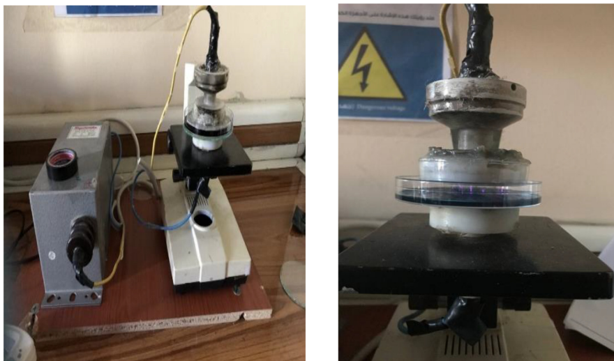
Fig. 1. High voltage Dielectric barrier discharge system.
