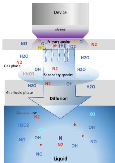
Fig. 6. Reactive species production in plasma discharge, gas phase, gas-liquid phase, and liquid phase represented graphically.
