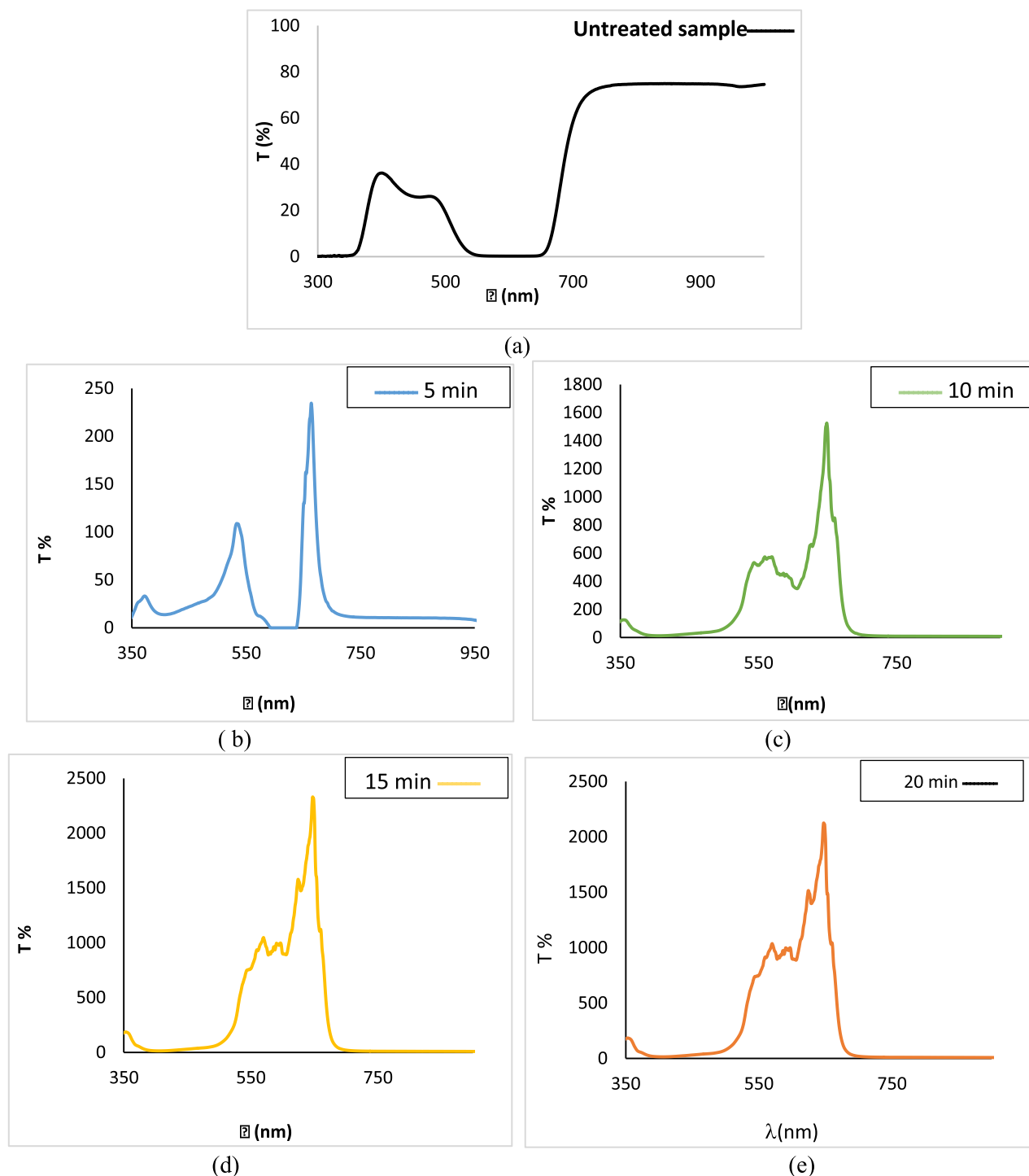
Fig. 4. The transmission of Indigo solution before and after exposed to cold plasma (a) untreated (b) 5 min. (c) 10 min. (d) 15 min. (e) 20 min.
