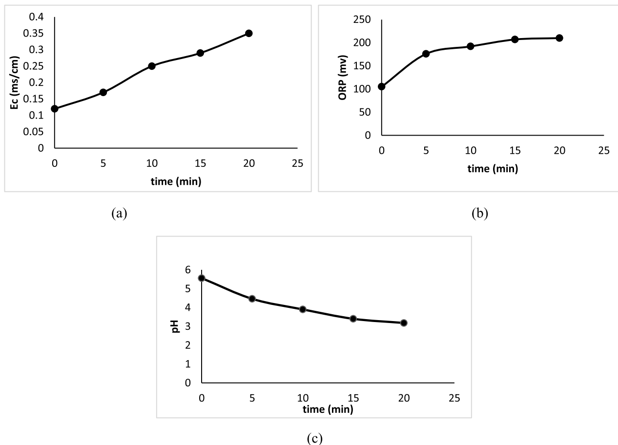
Fig. 3. Effect of cold plasma on (a), conductivity (b) ORP, (c) pH.
