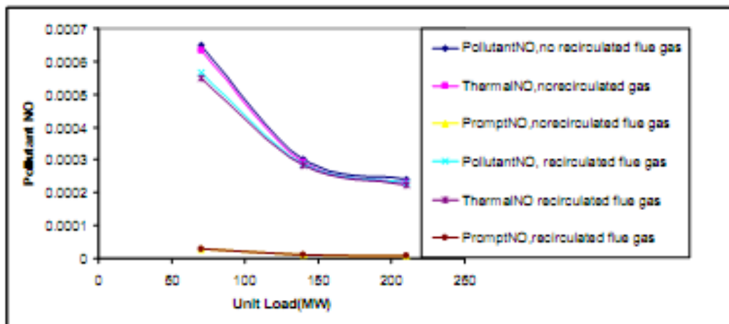
Figure (8) Pollutant NO for gaseous fuel with different load.
