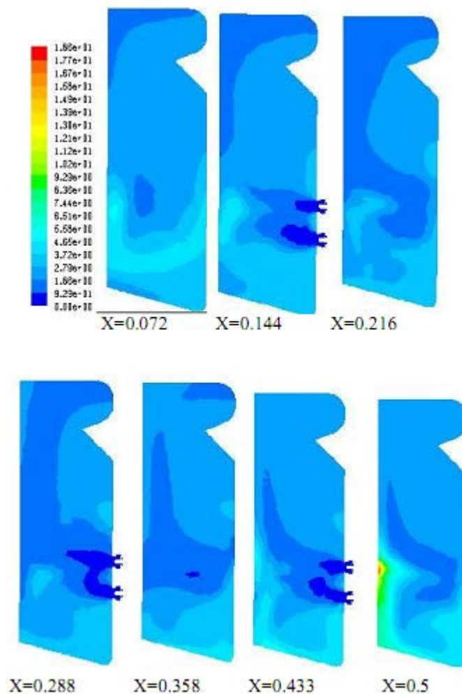
Figure (10) Contours of SOx for crude oil at different side planes
