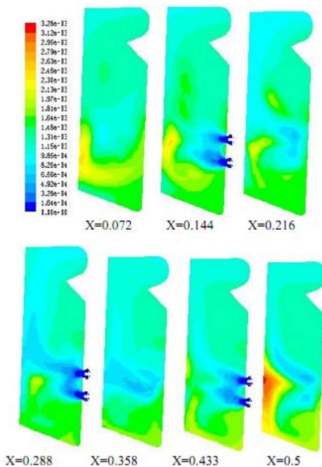
Figure (6) Contours of thermal NOx (crude oil) at different side planes.
