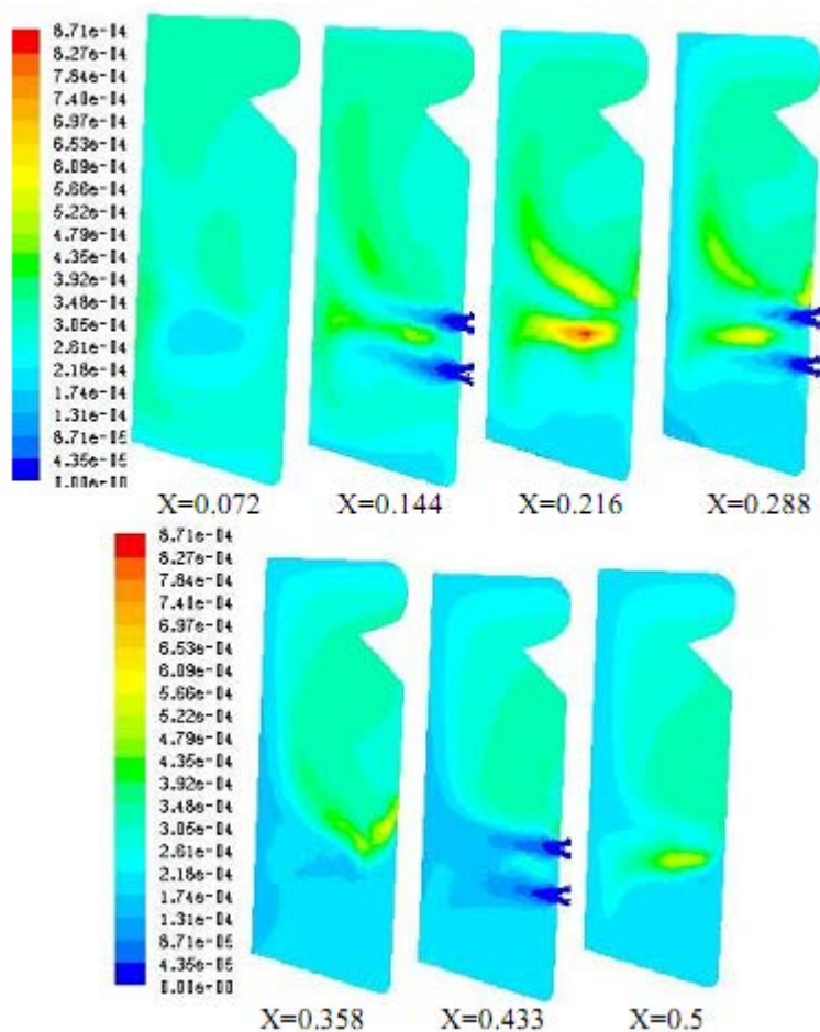
Figure (4) Contours of total pollutant of NO x (gaseous fuel)
