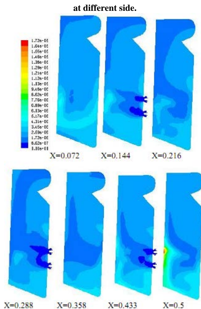
Figure (5) Contours of prompt NOx (crude oil) at different side planes.
