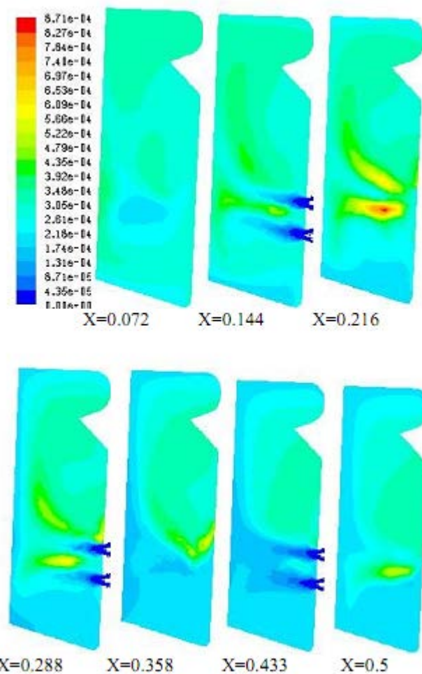
Figure (7) Contours of thermal NO x (gaseous fuel) at different side planes.
