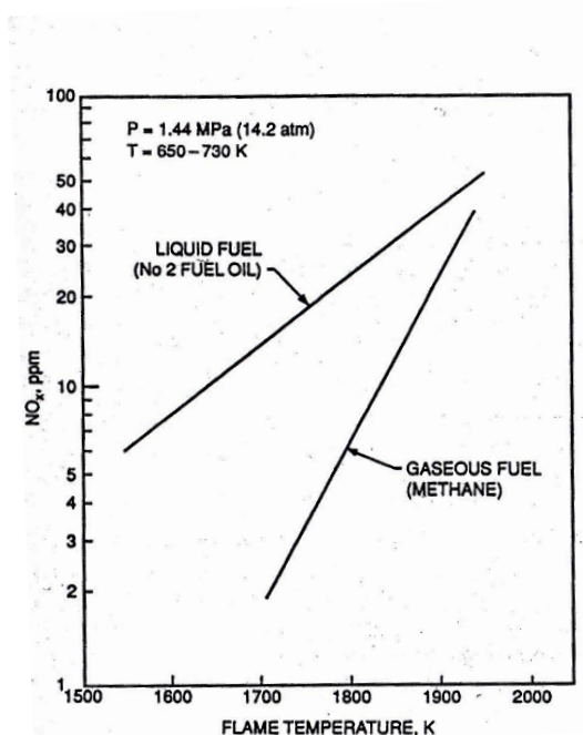
Figure (11) Dependence of \text{NO}_x on flame temperature for liquid and gaseous fuel [31].
