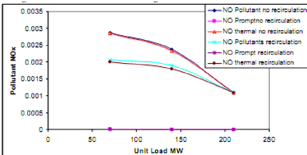
Figure (9) Pollutant NO for crude oil with different load.
