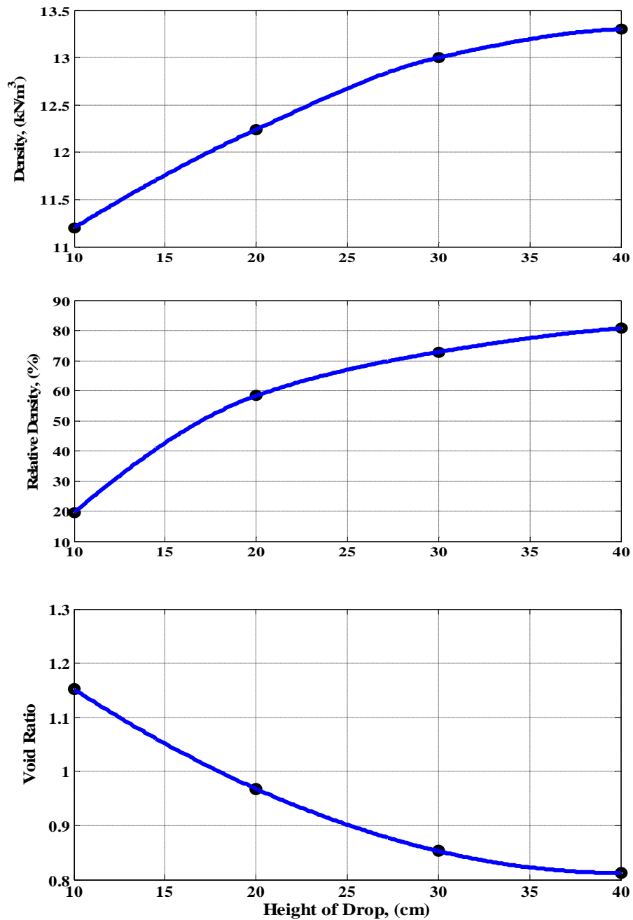
Figure (5) Density Calibration Curves for Gypsies Soil by Raining Technique.
