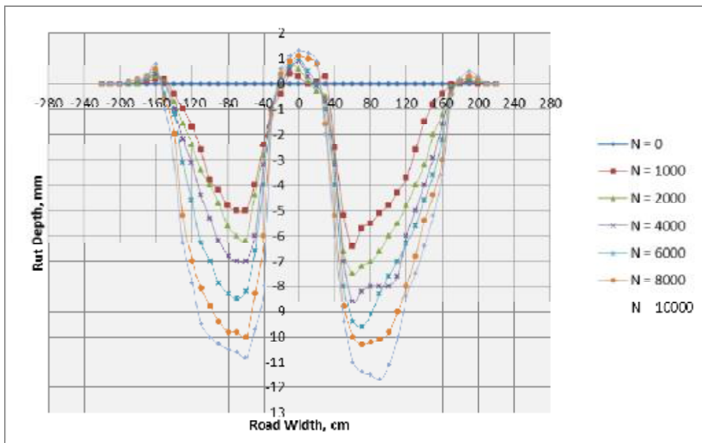
Figure (8) Rut Depth for Interfaces I+III.
