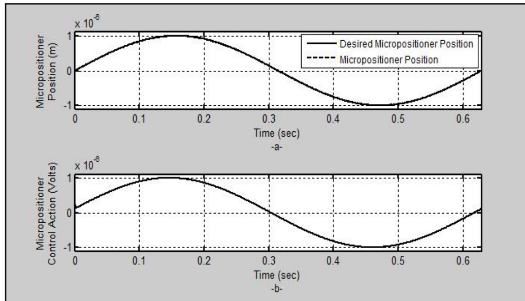
Figure (8) Simulation Results with sinusoidal input, magnitude= 1 \mu m , frequency= 10 \text{ rad/s} a- Time Response. b- Control Action.
