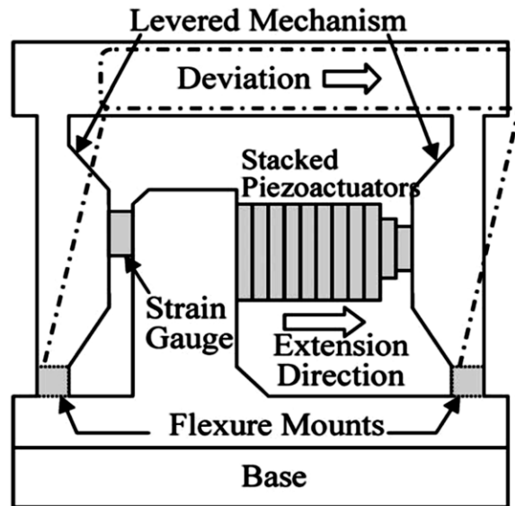
Figure (2) Working Principle of the Piezo-Positioning Stage [4].
