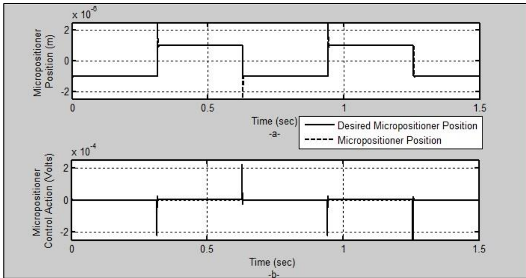
Figure (9) Simulation Results with square function input, magnitude= 1 \mu\text{m} , frequency=10 rad/s a- Time Response. b- Control Action.
