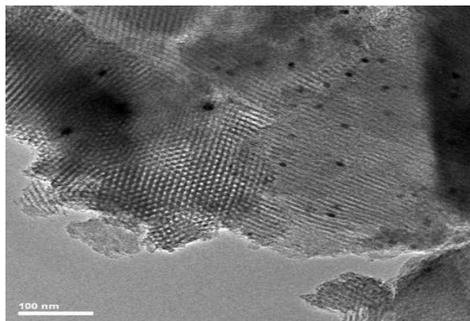
Figure (10) TEM images of 1% (Pt-Ni-Co)/SBA-15 at 100 nm.
