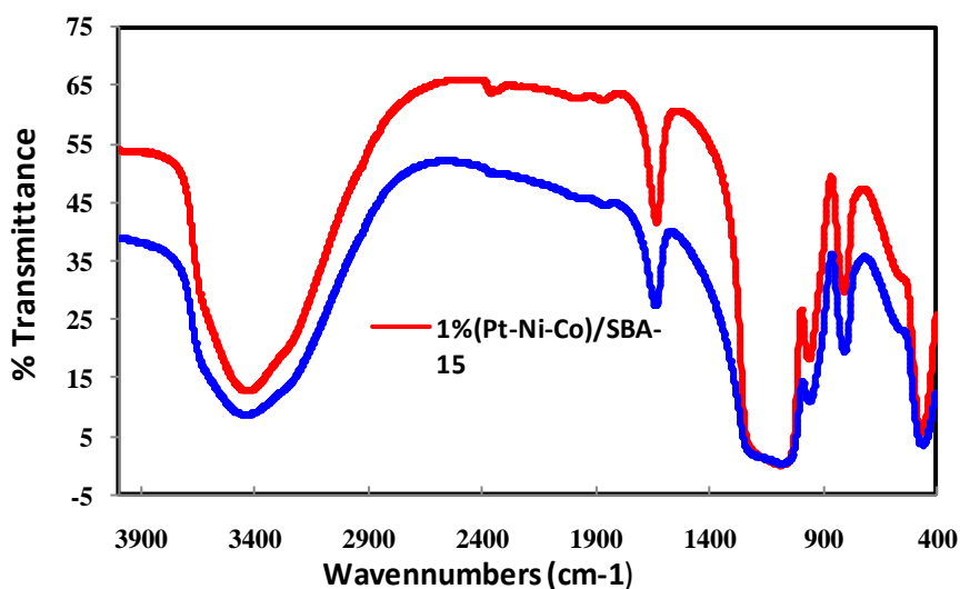
Figure (5) FT-IR spectra of SBA-15 and 1% (Pt-Ni-Co)/SBA-15.
