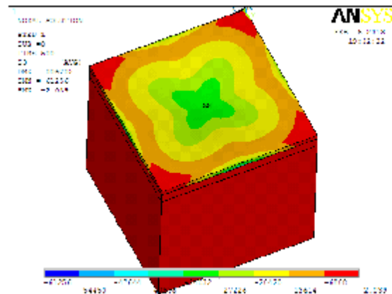
Figure (6) Contour Plot for 3 rd Principal Stress ( \sigma_3 ) (kN/m 2 ).
