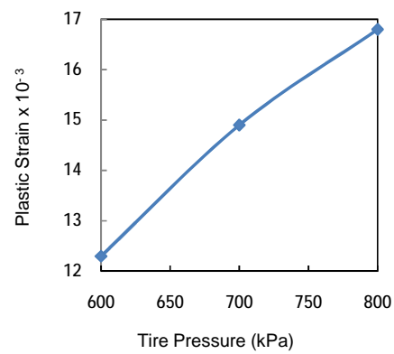
Figure (19) Variation of Plastic Strain with Pressure at T=50 °C.
