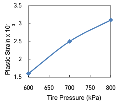
Figure (15) Variation of Plastic Strain With Pressure at T=20 °C .
