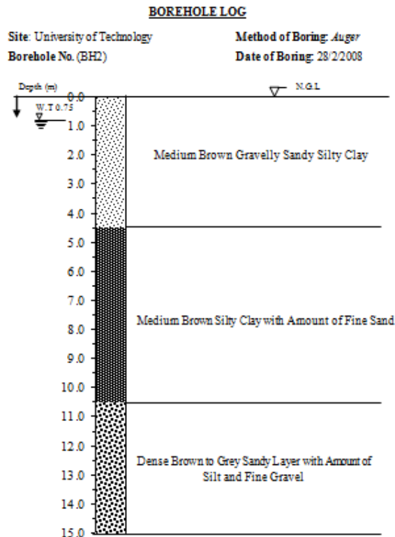
Figure (2) Stratigraphic column for the existed Borehole Within the site [8].
