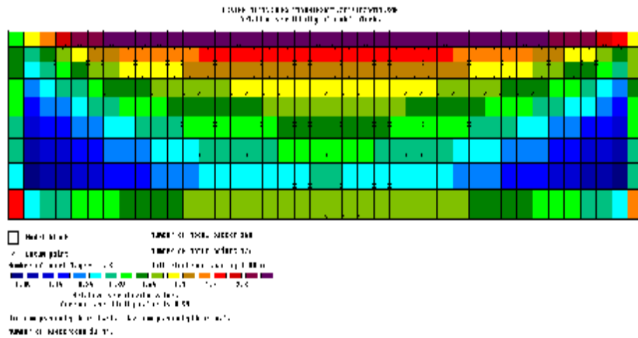
Figure (15) Block distribution generated by the sensitivity values of the model blocks for Wenner array.
