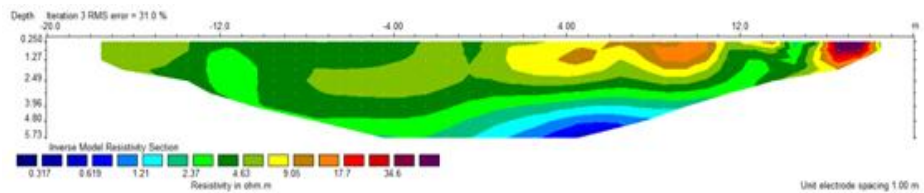
Figure (10) Resistivity section after extermination bad datum points.
