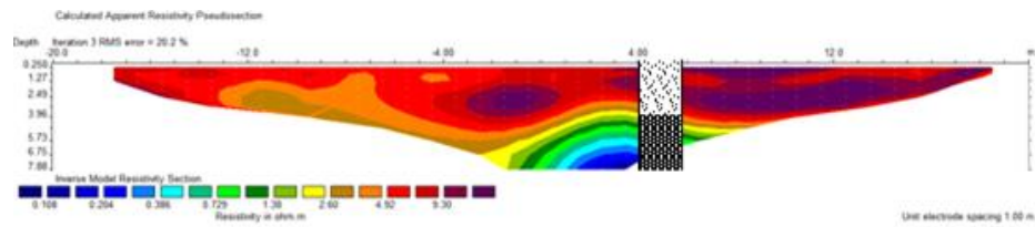
Figure (5) Correlation of inversion sections for the three arrays with the existed borehole and other features.
