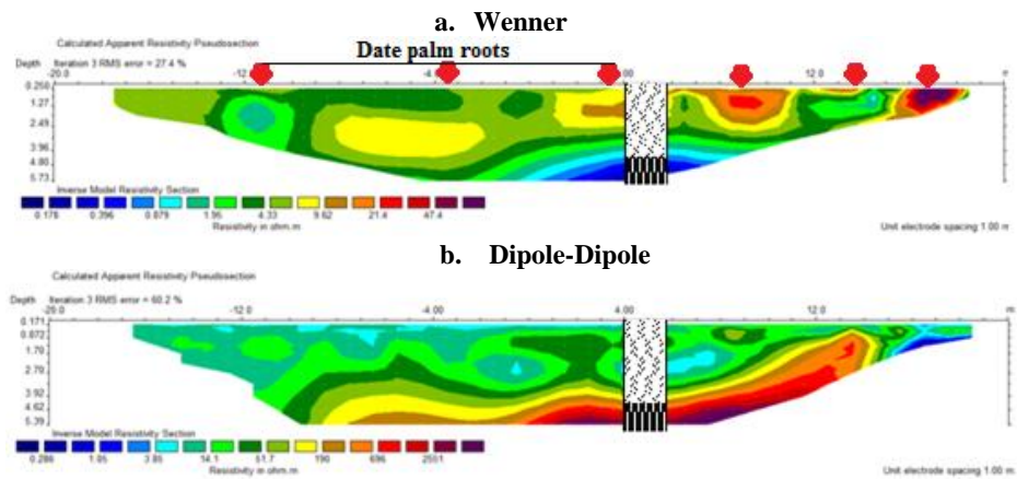
Figure (4) Inversion sections using Wenner, dipole-dipole and Wenner-Schlumberger arrays.
