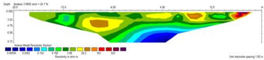
b. Dipole-Dipole
