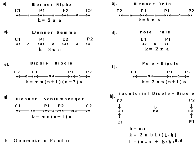
Figure (1) Common arrays used in resistivity surveys and Their geometric factors.
