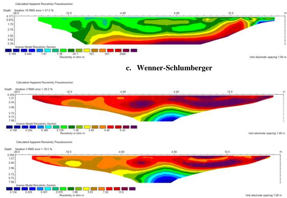
Figure (8) Inversion sections for the three arrays with different iterations.
