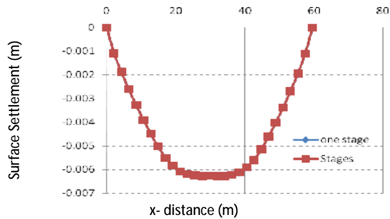
Figure (10 ) The effect of method of excavation on the surface Settlement due to excavation of tunnel 1 and tunnel 2.
