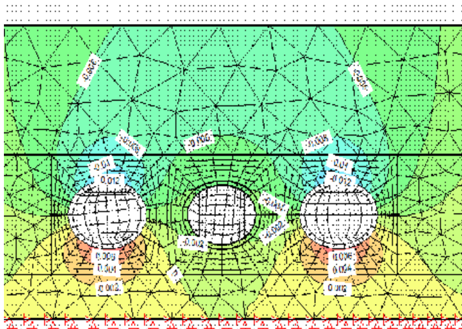
Figure (4) contour lines of vertical displacement using one stage in Excavation process.
