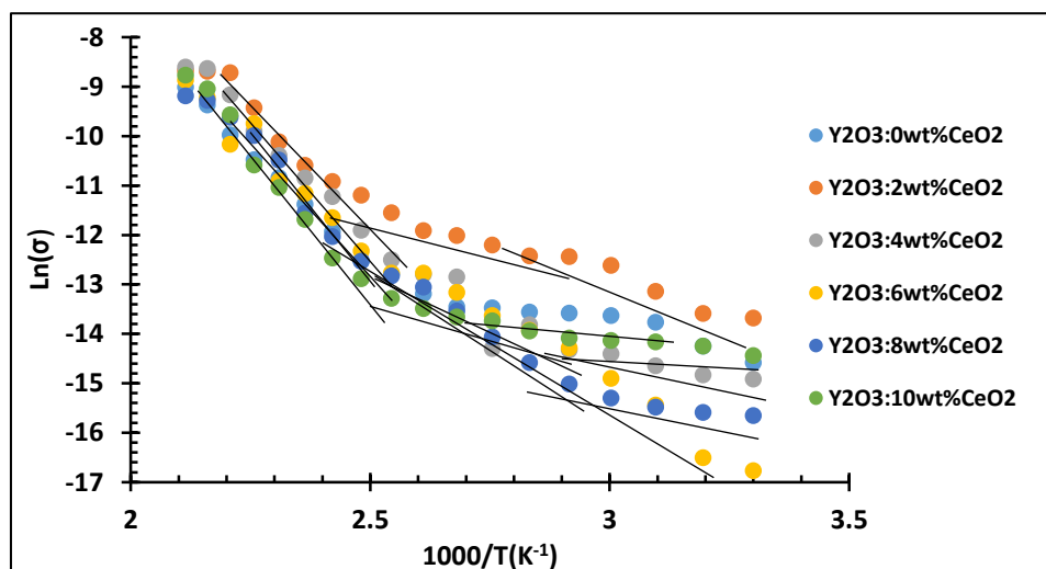
Figure 6- Variation of \ln(\sigma) with reciprocal temperature for Y_2O_3 doped with CeO_2 at different doping ratios
