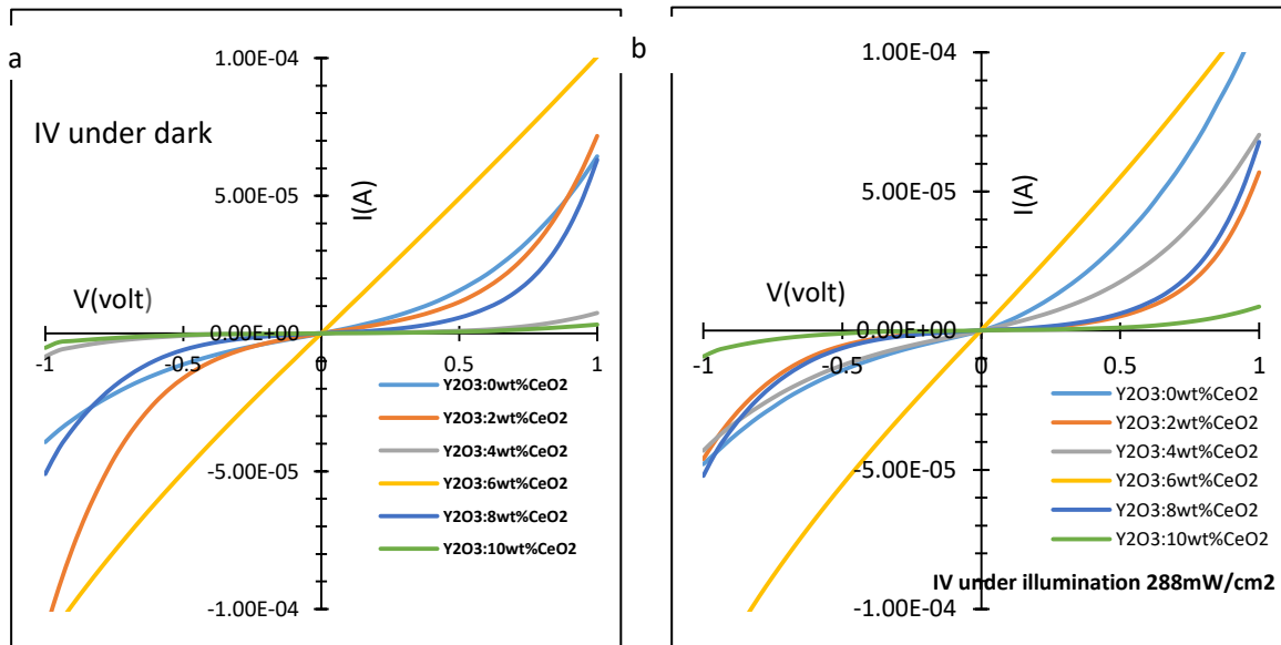
Figure 7- I-V characteristic curves (a) under dark and (b) illumination for undoped Y_2O_3 and doped with different ratios of CeO_2 films.
