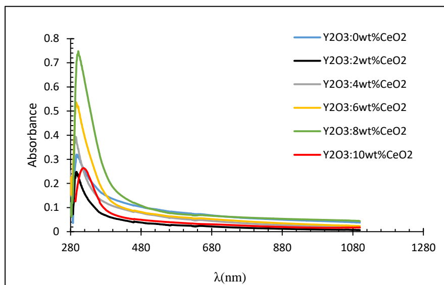
Figure 3- Absorbance spectra for undoped \text{Y}_2\text{O}_3 film and doped with (2, 4, 6, 8, and 10)%wt. \text{CeO}_2 .
