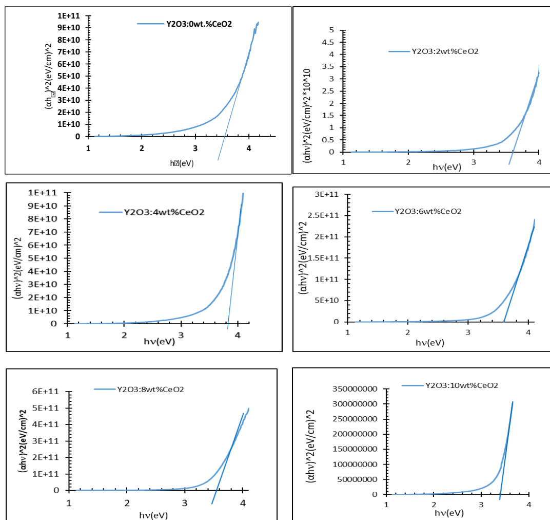
Figure 4- (\alpha h\nu)^2 vs. (h\nu) plots for undoped \text{Y}_2\text{O}_3 and doped with (2, 4, 6, 8, 10)wt.% \text{CeO}_2 films
