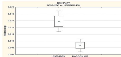
Figure 1. Box Charts: Comparison of Weight Loss Between S355J2G3 and HARDOX 450 Materials
