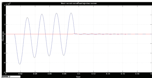
Fig. (10): The current of short circuit and the current of injection for one phase.
