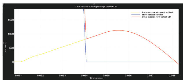
Fig. (18): The magnifier graphic for injected current, short circuit current and the total current flow through tested CB.
