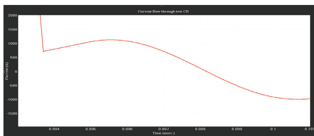
Fig. (17): The magnifier view for injection current flow through tested CB.
