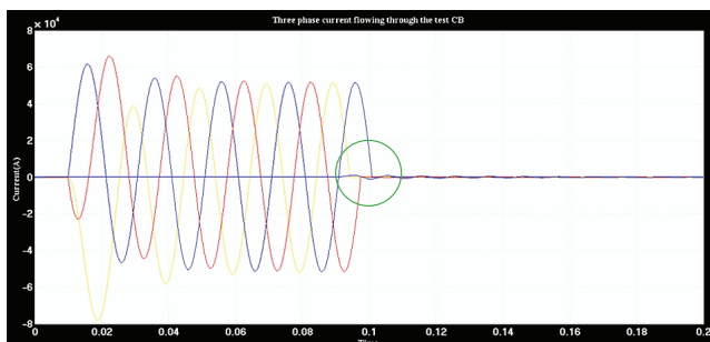
Fig. (16): Current of short circuit, the injection current, and the current will flowing through the tested C.B.
