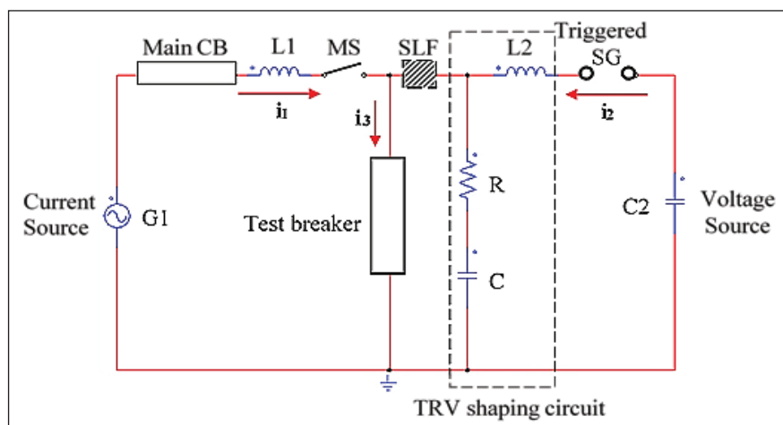
Fig. (2): Proposed circuit of parallel current injection for a CB test circuit.
