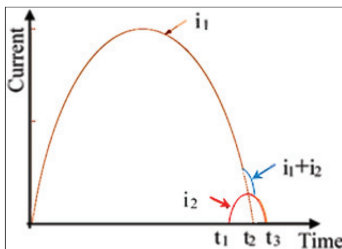
Fig. (3): The relation of the current at short circuit and the current flow from DC source [8].
