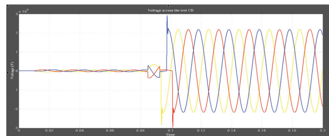
Fig. (12): Voltage waveform across the test C.B before and after the interrupting.
