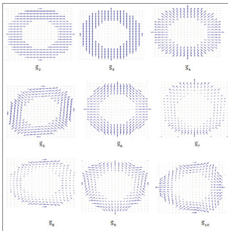
Fig. (1): Plots of first (9) orthonormal annular vector ZPs', ( S^{\sim} ), with ( \epsilon=0.2 )
