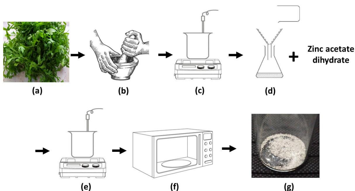
Fig. 1: Illustrates the process of producing zinc oxide nanoparticles (ZnO NPs) from Lepidium sativum L. leaves. (a) It involves washing the leaves, (b) Crushing them with a mortar and pestle, (c) Mixing the paste with distilled water and heating it at 70°C, (d) Filtering the product, combining it with zinc acetate dihydrate, (e) Heating and stirring until it forms a paste, (f) Burning the paste at 350°C, and (g) Finally obtaining the ZnO NPs powder.
